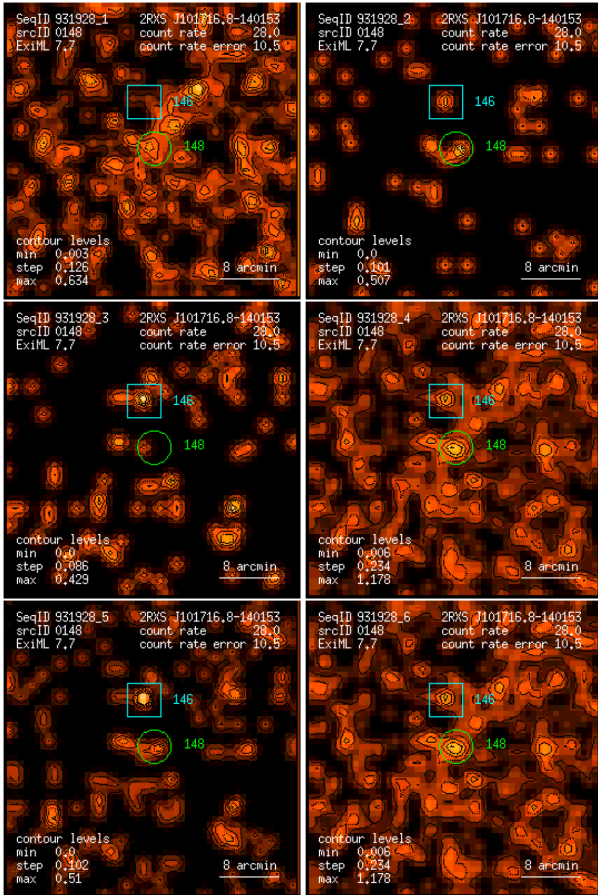
Figure 148: RASS 931928: detection 0148: band rate images, Gaussian filter: (1) PSPC channels 11 – 41, (2) 52 – 90, (3) 91 – 201, (4) 11 – 235, (5) 52 – 201, (6) 11 – 201. Broad band rates in counts/ks. Band rate contour levels in counts/ks/arcmin 2 .
