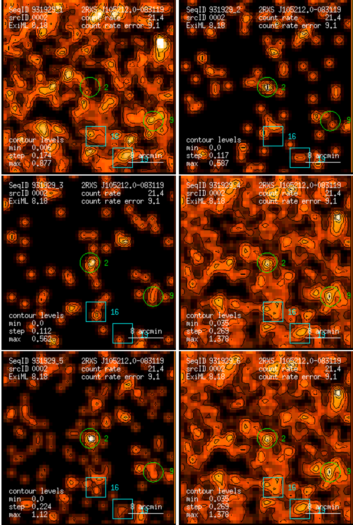
Figure 2: RASS 931929: detection 0002: band rate images, Gaussian filter: (1) PSPC channels 11 – 41, (2) 52 – 90, (3) 91 – 201, (4) 11 – 235, (5) 52 – 201, (6) 11 – 201. Broad band rates in counts/ks. Band rate contour levels in counts/ks/arcmin 2 .
