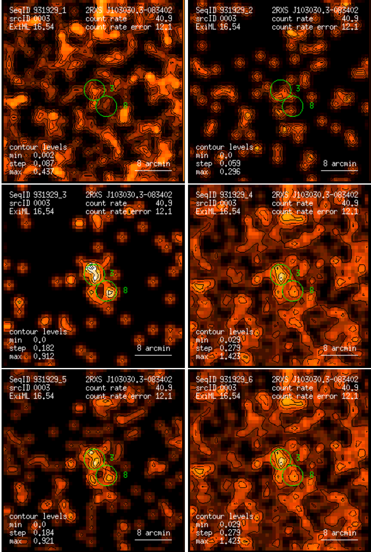
Figure 3: RASS 931929: detection 0003: band rate images, Gaussian filter: (1) PSPC channels 11 – 41, (2) 52 – 90, (3) 91 – 201, (4) 11 – 235, (5) 52 – 201, (6) 11 – 201. Broad band rates in counts/ks. Band rate contour levels in counts/ks/arcmin 2 .
