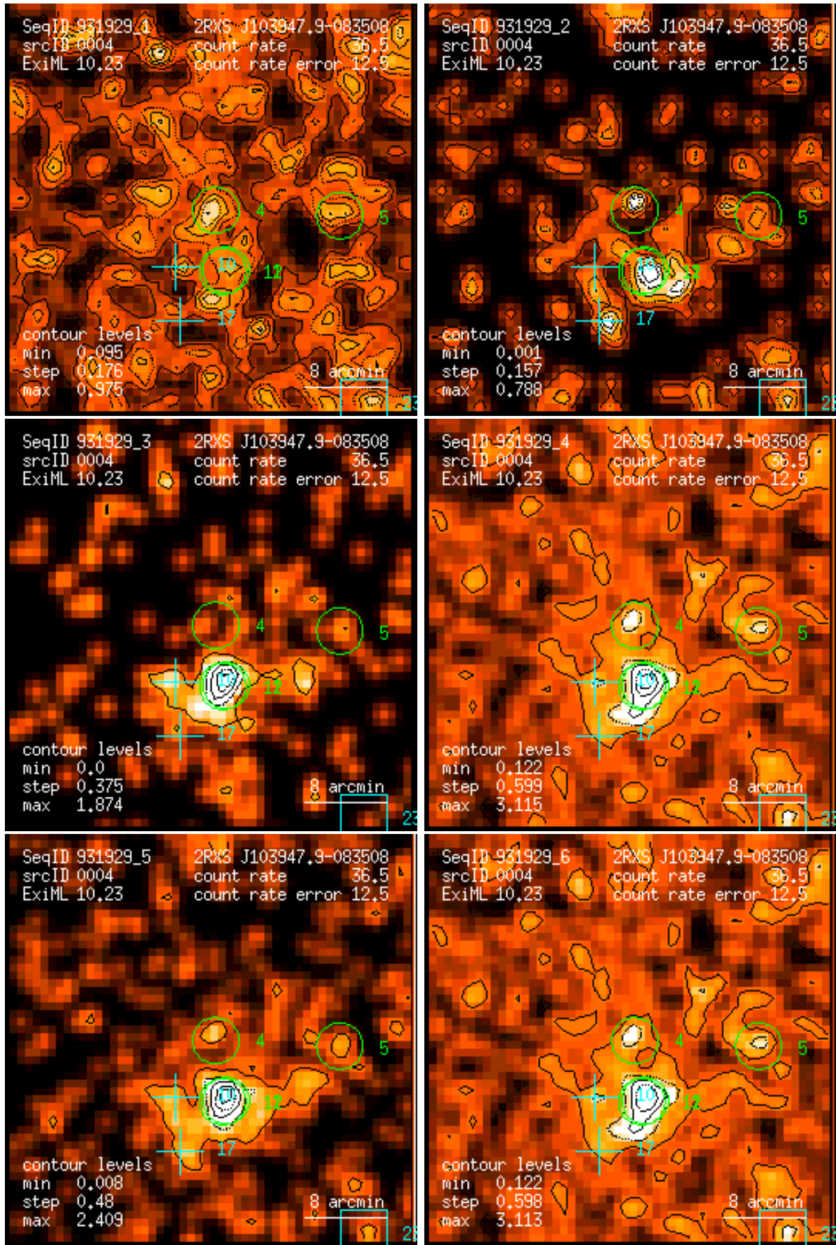
Figure 4: RASS 931929: detection 0004: band rate images, Gaussian filter: (1) PSPC channels 11 – 41, (2) 52 – 90, (3) 91 – 201, (4) 11 – 235, (5) 52 – 201, (6) 11 – 201. Broad band rates in counts/ks. Band rate contour levels in counts/ks/arcmin 2 .
