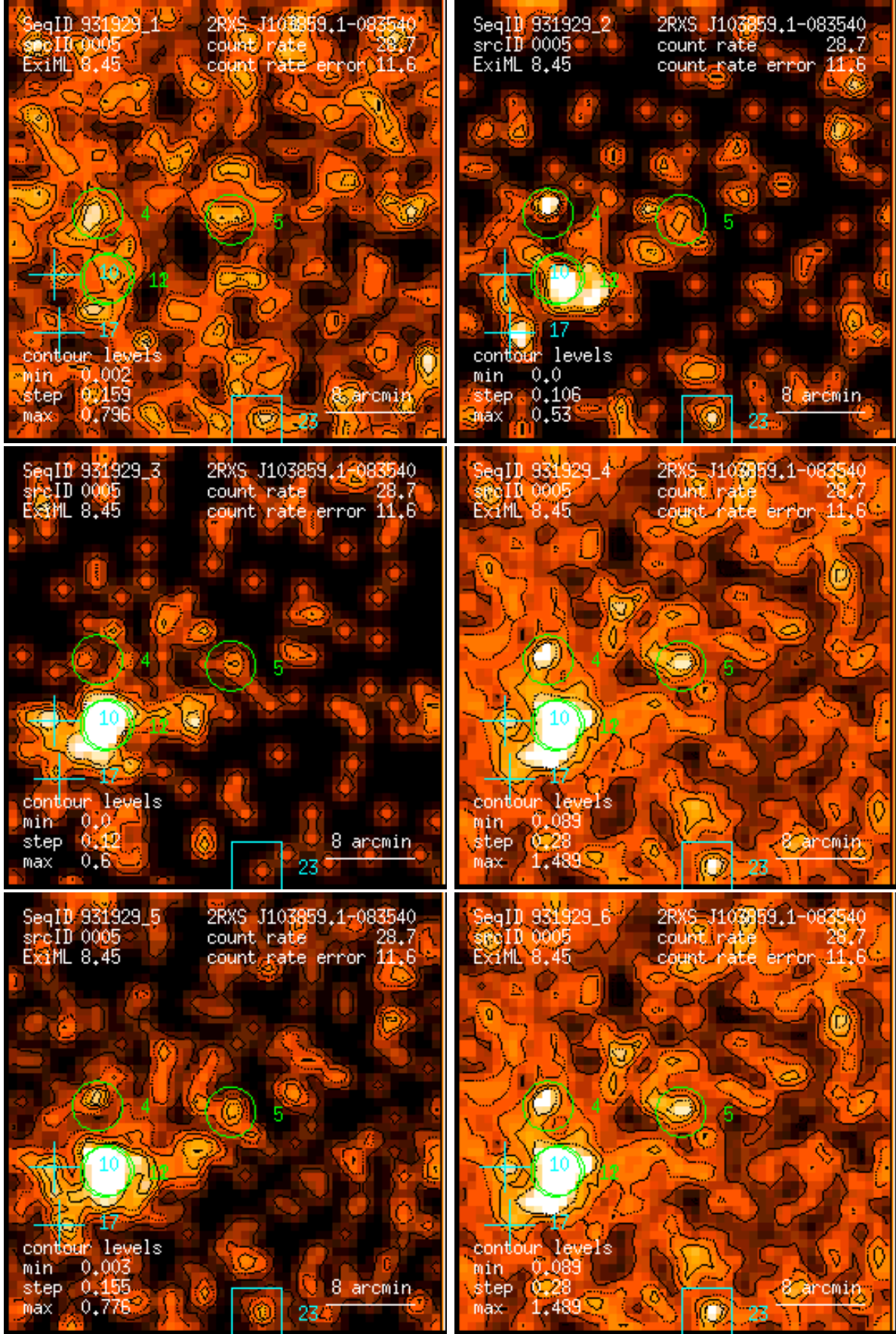
Figure 5: RASS 931929: detection 0005: band rate images, Gaussian filter: (1) PSPC channels 11 – 41, (2) 52 – 90, (3) 91 – 201, (4) 11 – 235, (5) 52 – 201, (6) 11 – 201. Broad band rates in counts/ks. Band rate contour levels in counts/ks/arcmin 2 .
