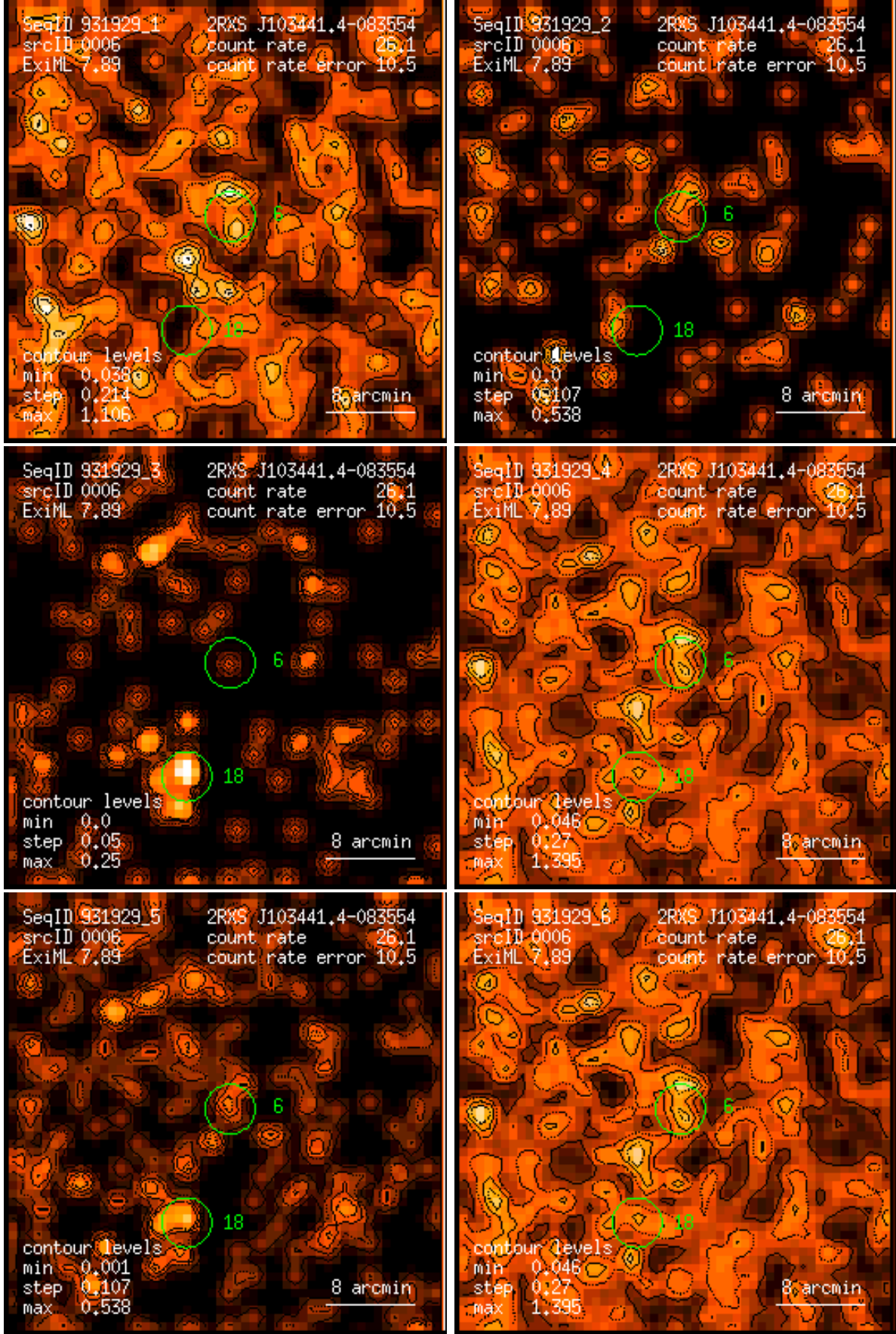
Figure 6: RASS 931929: detection 0006: band rate images, Gaussian filter: (1) PSPC channels 11 – 41, (2) 52 – 90, (3) 91 – 201, (4) 11 – 235, (5) 52 – 201, (6) 11 – 201. Broad band rates in counts/ks. Band rate contour levels in counts/ks/arcmin 2 .
