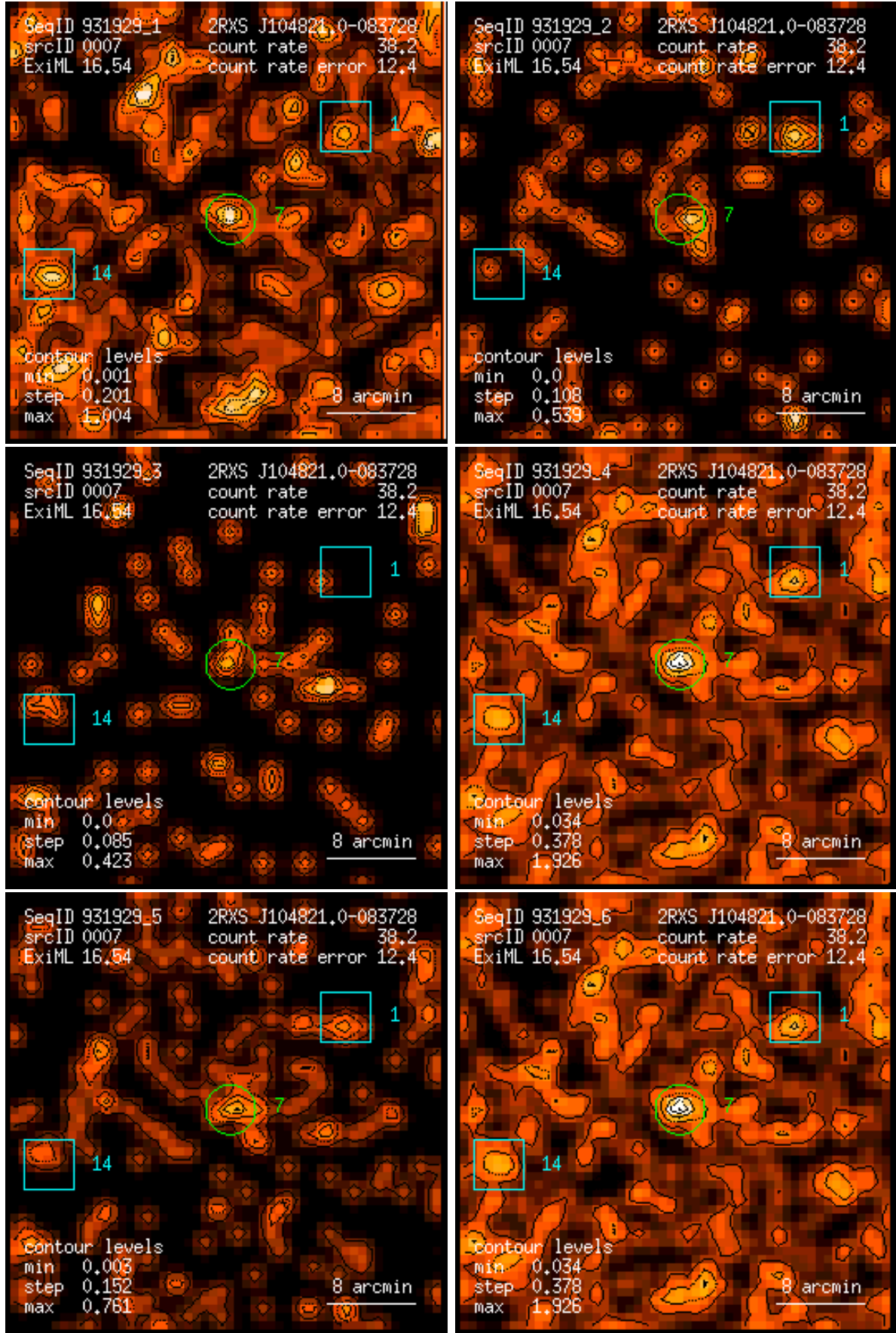
Figure 7: RASS 931929: detection 0007: band rate images, Gaussian filter: (1) PSPC channels 11 – 41, (2) 52 – 90, (3) 91 – 201, (4) 11 – 235, (5) 52 – 201, (6) 11 – 201. Broad band rates in counts/ks. Band rate contour levels in counts/ks/arcmin 2 .
