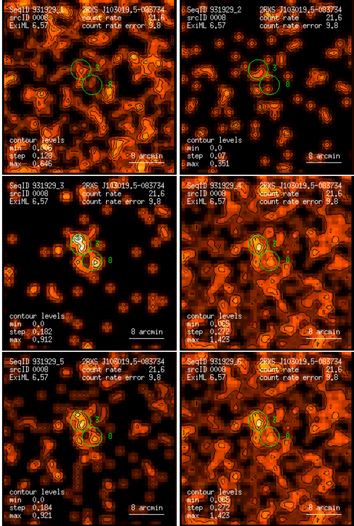
Figure 8: RASS 931929: detection 0008: band rate images, Gaussian filter: (1) PSPC channels 11 – 41, (2) 52 – 90, (3) 91 – 201, (4) 11 – 235, (5) 52 – 201, (6) 11 – 201. Broad band rates in counts/ks. Band rate contour levels in counts/ks/arcmin 2 .
