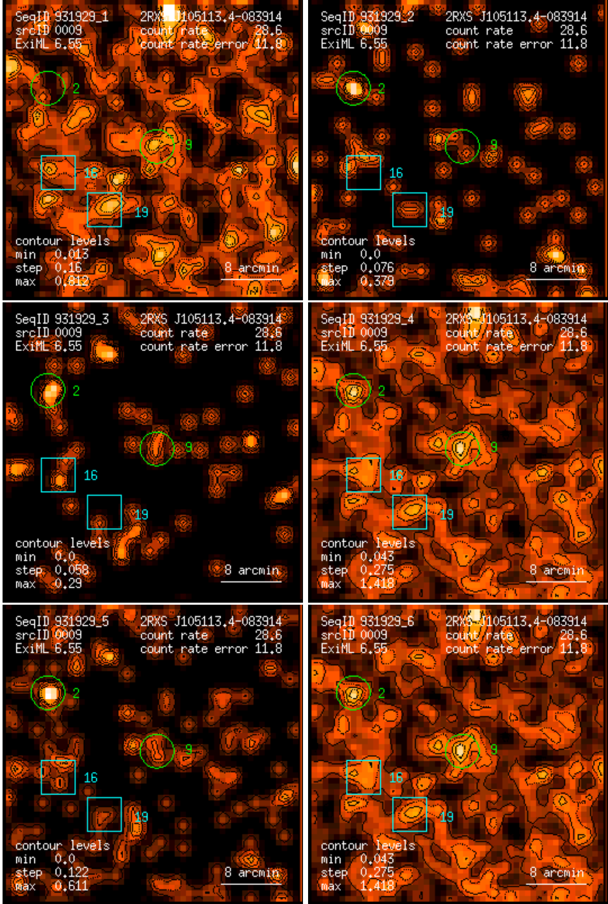
Figure 9: RASS 931929: detection 0009: band rate images, Gaussian filter: (1) PSPC channels 11 – 41, (2) 52 – 90, (3) 91 – 201, (4) 11 – 235, (5) 52 – 201, (6) 11 – 201. Broad band rates in counts/ks. Band rate contour levels in counts/ks/arcmin 2 .
