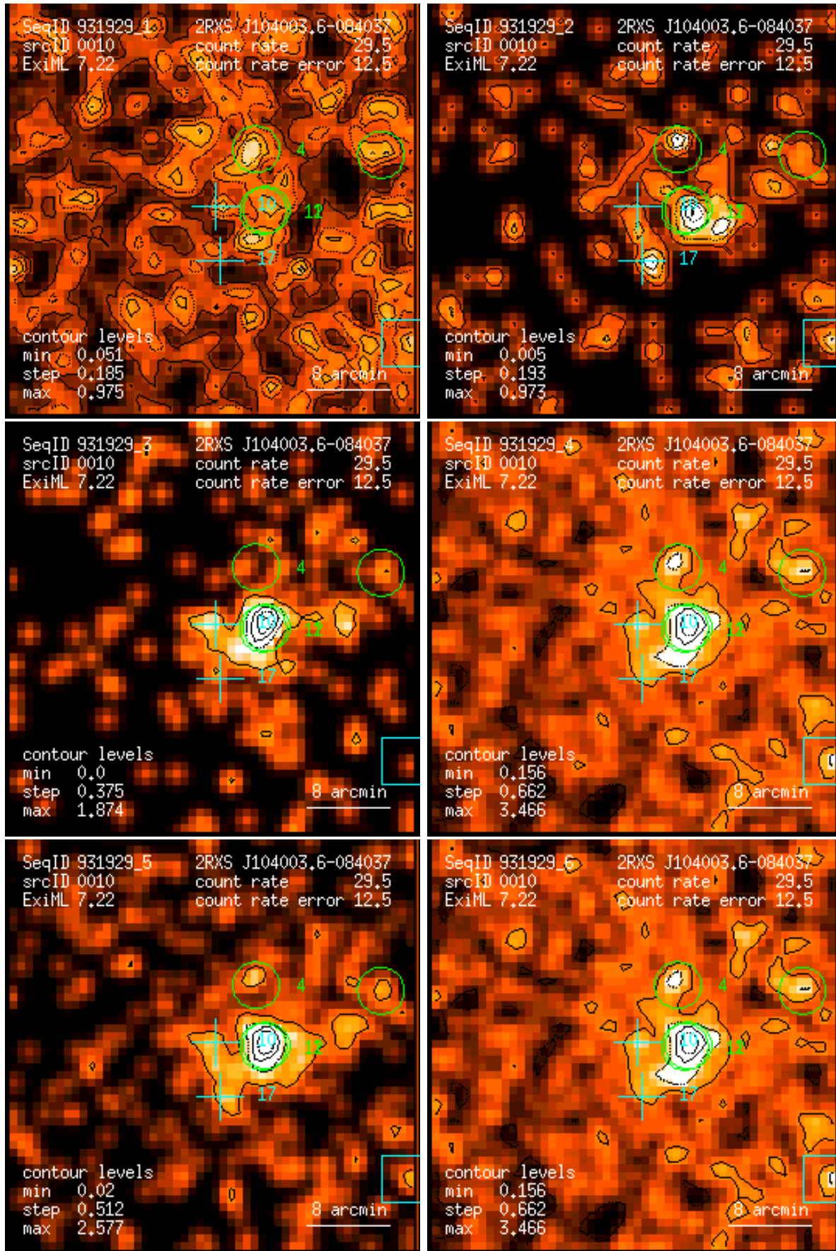
Figure 10: RASS 931929: detection 0010: band rate images, Gaussian filter: (1) PSPC channels 11 – 41, (2) 52 – 90, (3) 91 – 201, (4) 11 – 235, (5) 52 – 201, (6) 11 – 201. Broad band rates in counts/ks. Band rate contour levels in counts/ks/arcmin 2 .
