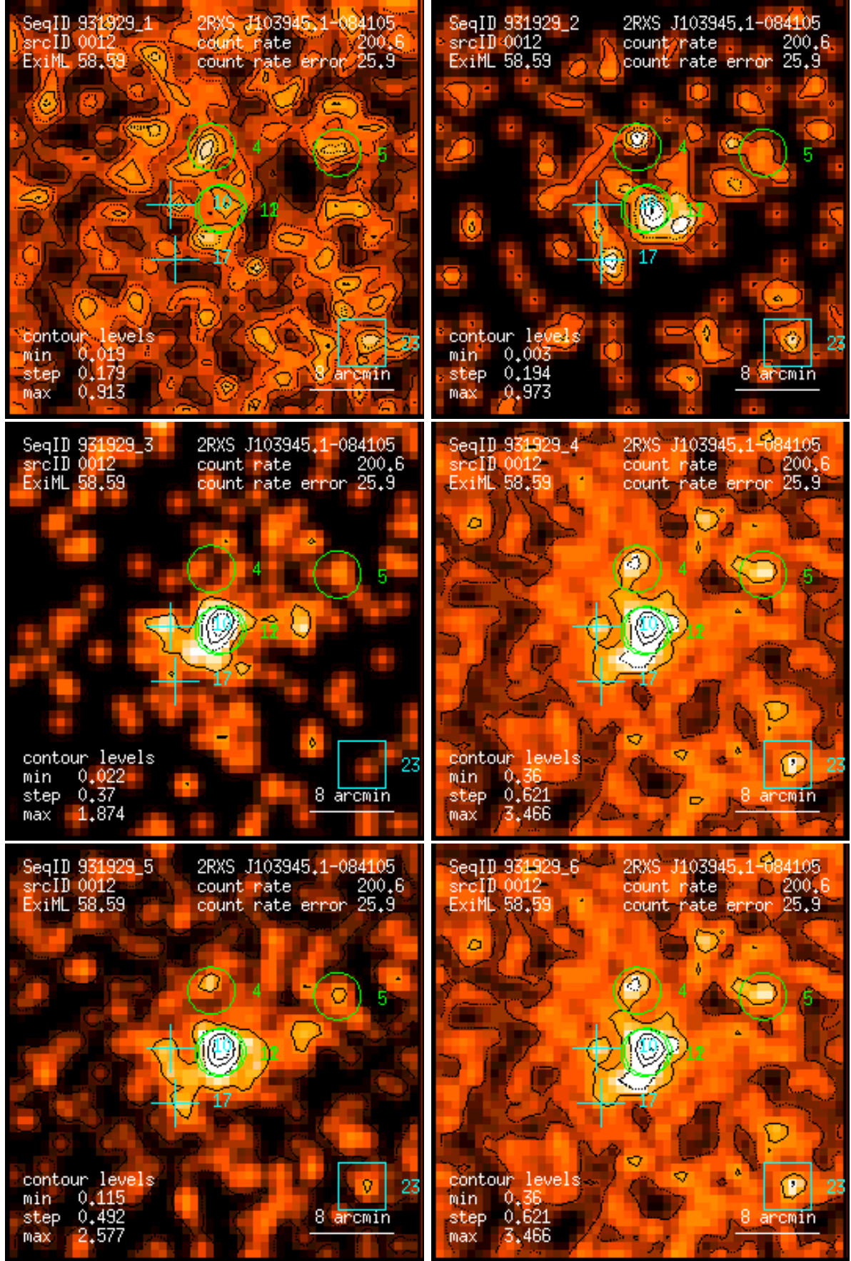
Figure 12: RASS 931929: detection 0012: band rate images, Gaussian filter: (1) PSPC channels 11 – 41, (2) 52 – 90, (3) 91 – 201, (4) 11 – 235, (5) 52 – 201, (6) 11 – 201. Broad band rates in counts/ks. Band rate contour levels in counts/ks/arcmin 2 .
