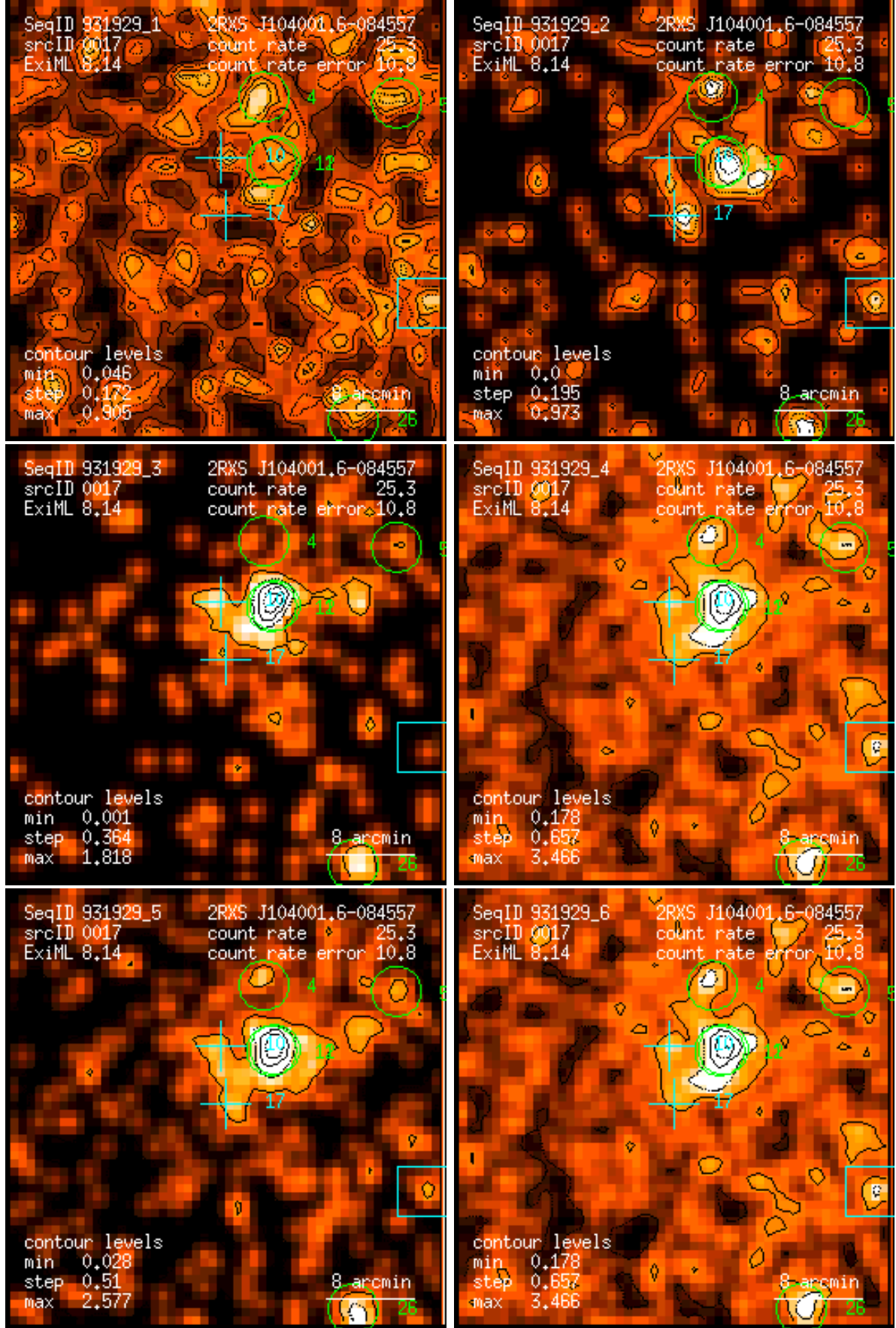
Figure 17: RASS 931929: detection 0017: band rate images, Gaussian filter: (1) PSPC channels 11 – 41, (2) 52 – 90, (3) 91 – 201, (4) 11 – 235, (5) 52 – 201, (6) 11 – 201. Broad band rates in counts/ks. Band rate contour levels in counts/ks/arcmin 2 .
