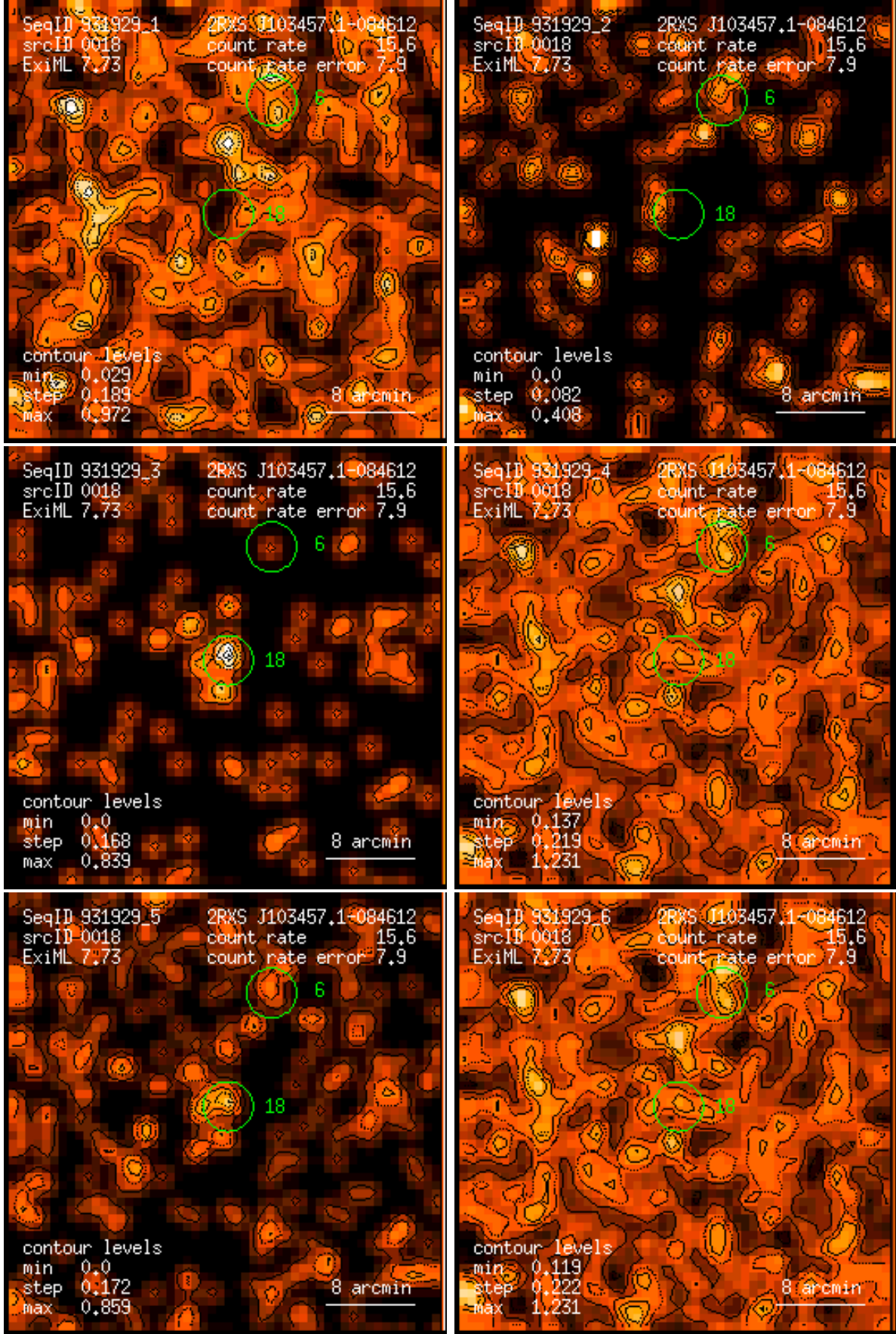
Figure 18: RASS 931929: detection 0018: band rate images, Gaussian filter: (1) PSPC channels 11 – 41, (2) 52 – 90, (3) 91 – 201, (4) 11 – 235, (5) 52 – 201, (6) 11 – 201. Broad band rates in counts/ks. Band rate contour levels in counts/ks/arcmin 2 .
