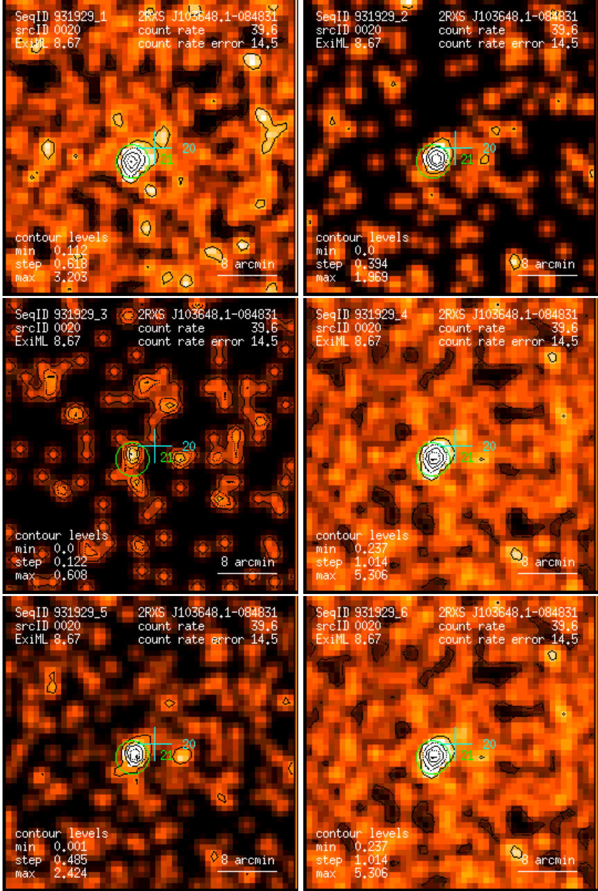
Figure 20: RASS 931929: detection 0020: band rate images, Gaussian filter: (1) PSPC channels 11 – 41, (2) 52 – 90, (3) 91 – 201, (4) 11 – 235, (5) 52 – 201, (6) 11 – 201. Broad band rates in counts/ks. Band rate contour levels in counts/ks/arcmin 2 .
