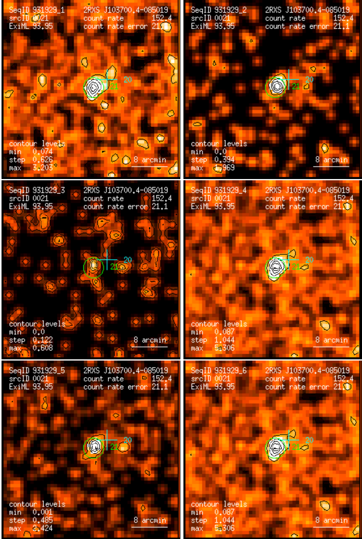
Figure 21: RASS 931929: detection 0021: band rate images, Gaussian filter: (1) PSPC channels 11 – 41, (2) 52 – 90, (3) 91 – 201, (4) 11 – 235, (5) 52 – 201, (6) 11 – 201. Broad band rates in counts/ks. Band rate contour levels in counts/ks/arcmin 2 .
