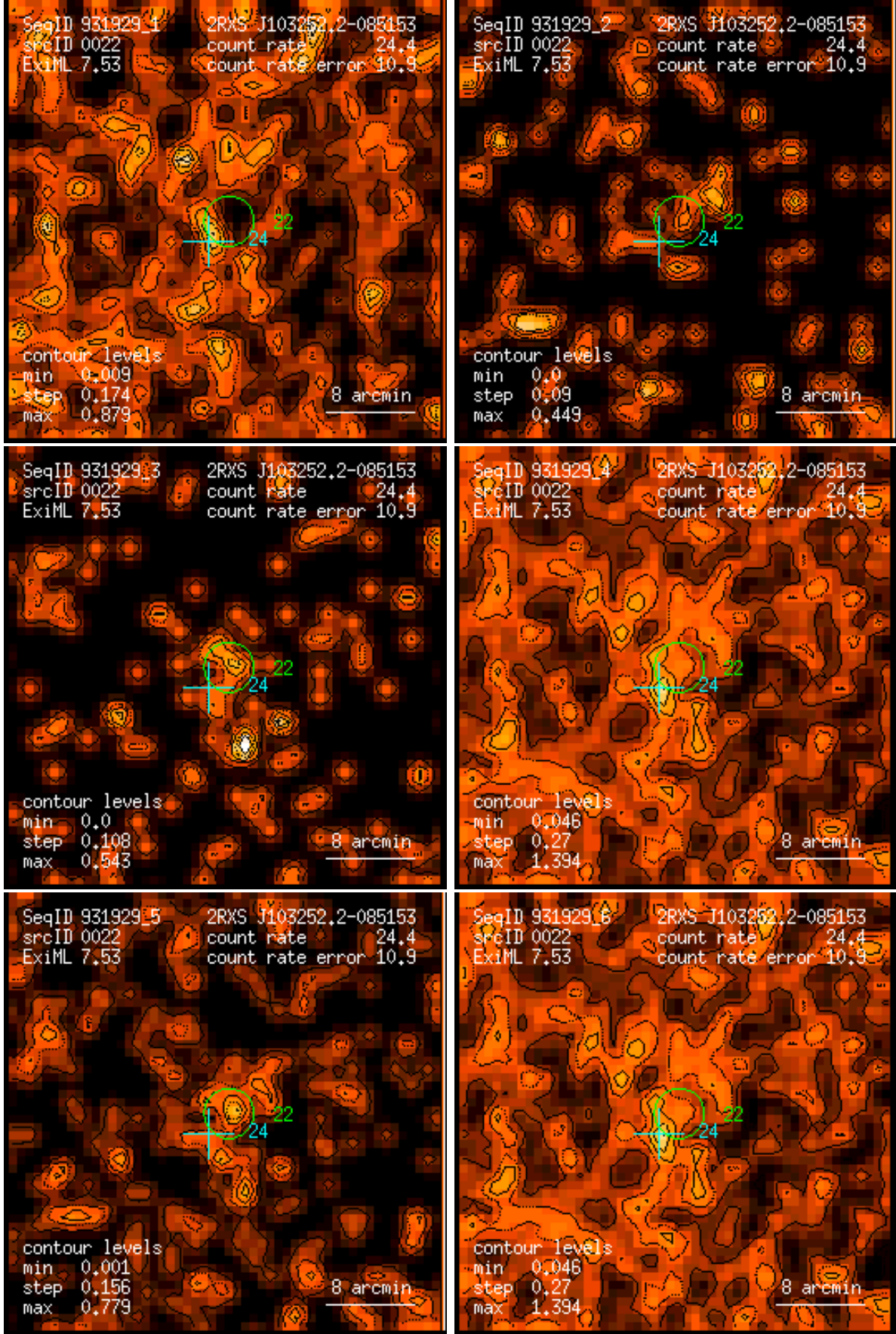
Figure 22: RASS 931929: detection 0022: band rate images, Gaussian filter: (1) PSPC channels 11 – 41, (2) 52 – 90, (3) 91 – 201, (4) 11 – 235, (5) 52 – 201, (6) 11 – 201. Broad band rates in counts/ks. Band rate contour levels in counts/ks/arcmin 2 .
