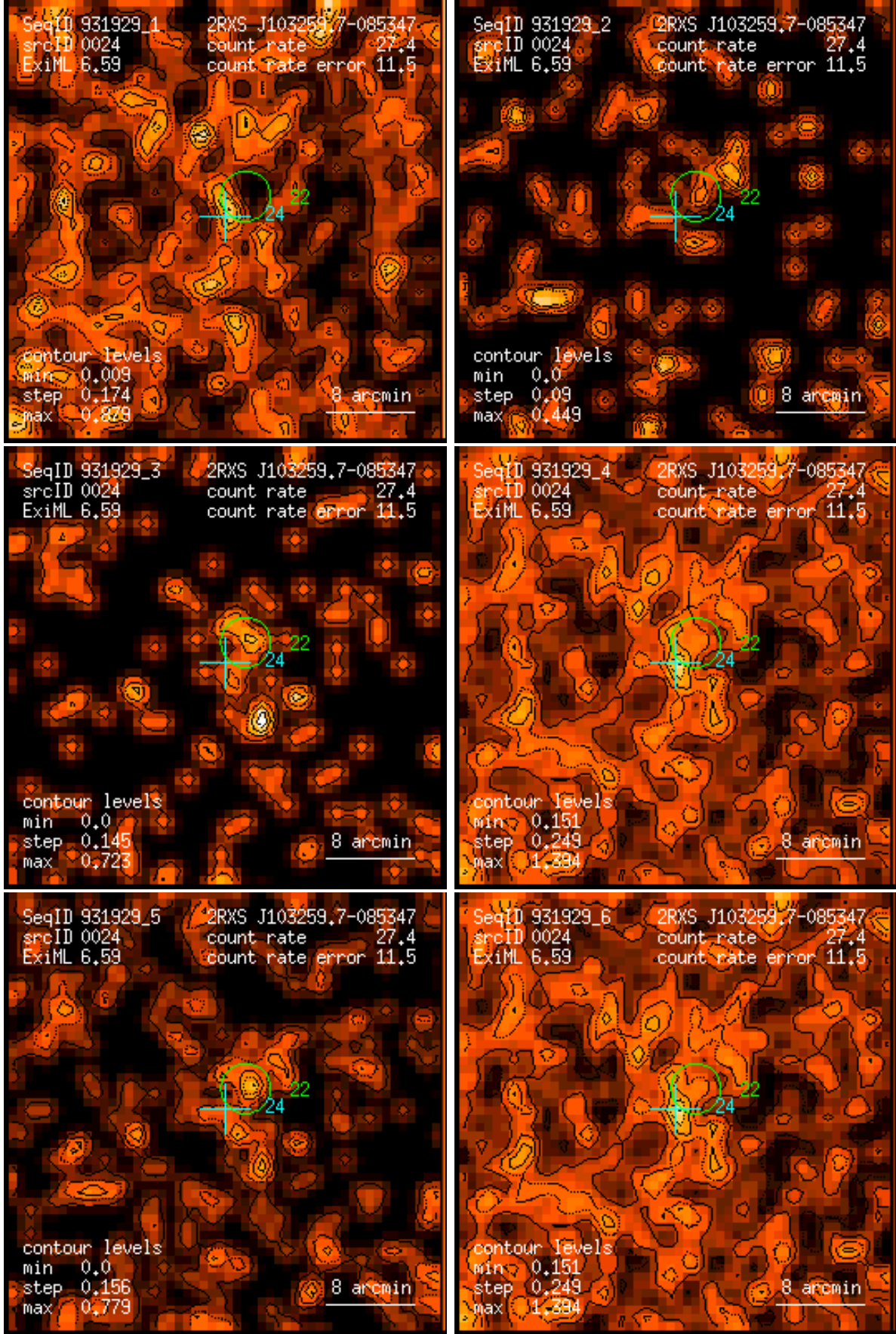
Figure 24: RASS 931929: detection 0024: band rate images, Gaussian filter: (1) PSPC channels 11 – 41, (2) 52 – 90, (3) 91 – 201, (4) 11 – 235, (5) 52 – 201, (6) 11 – 201. Broad band rates in counts/ks. Band rate contour levels in counts/ks/arcmin 2 .
