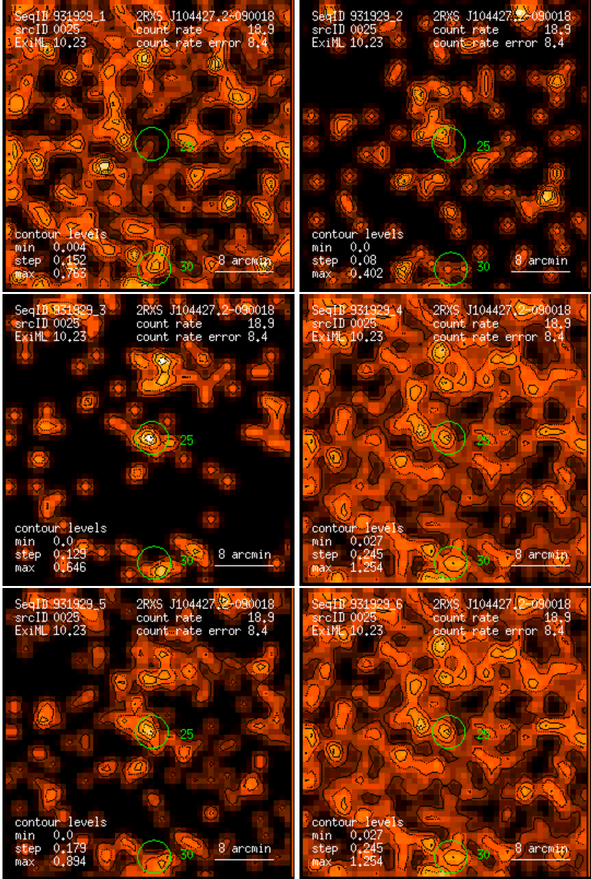
Figure 25: RASS 931929: detection 0025: band rate images, Gaussian filter: (1) PSPC channels 11 – 41, (2) 52 – 90, (3) 91 – 201, (4) 11 – 235, (5) 52 – 201, (6) 11 – 201. Broad band rates in counts/ks. Band rate contour levels in counts/ks/arcmin 2 .
