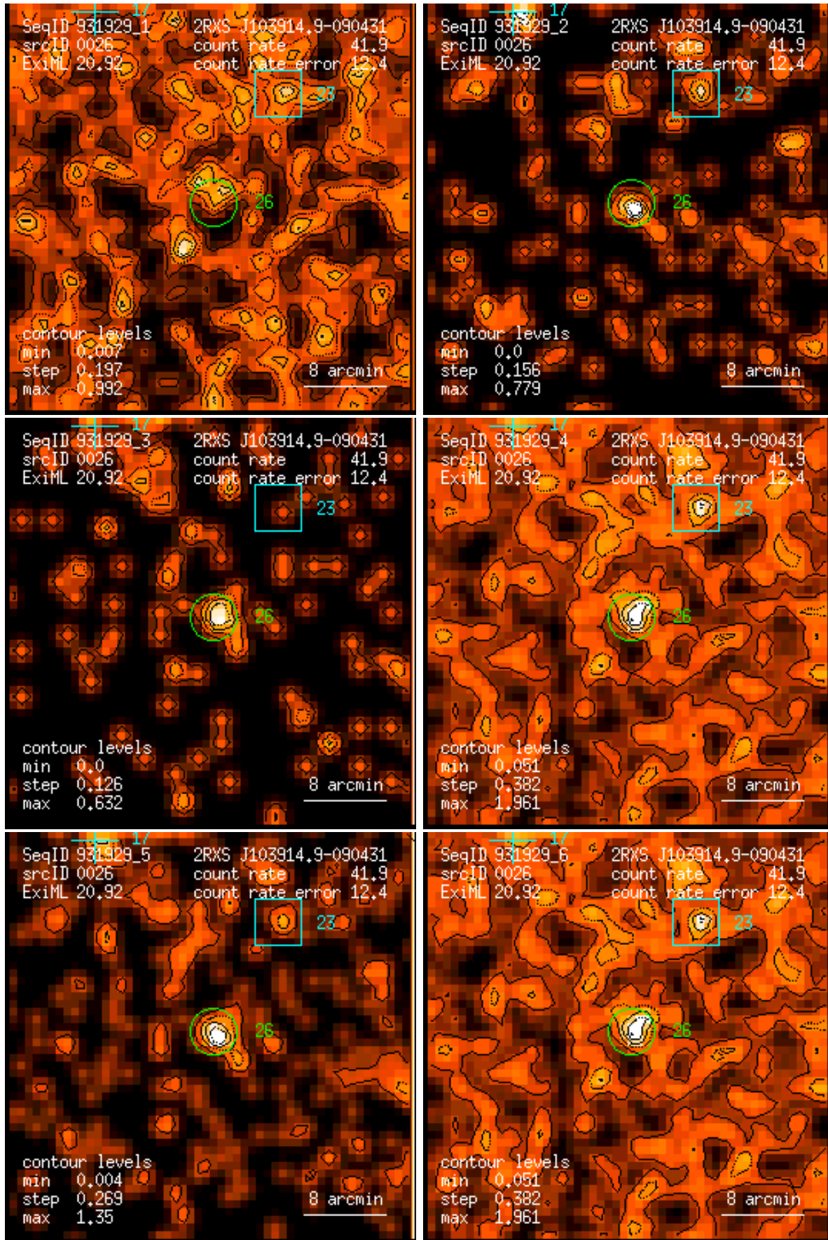
Figure 26: RASS 931929: detection 0026: band rate images, Gaussian filter: (1) PSPC channels 11 – 41, (2) 52 – 90, (3) 91 – 201, (4) 11 – 235, (5) 52 – 201, (6) 11 – 201. Broad band rates in counts/ks. Band rate contour levels in counts/ks/arcmin 2 .
