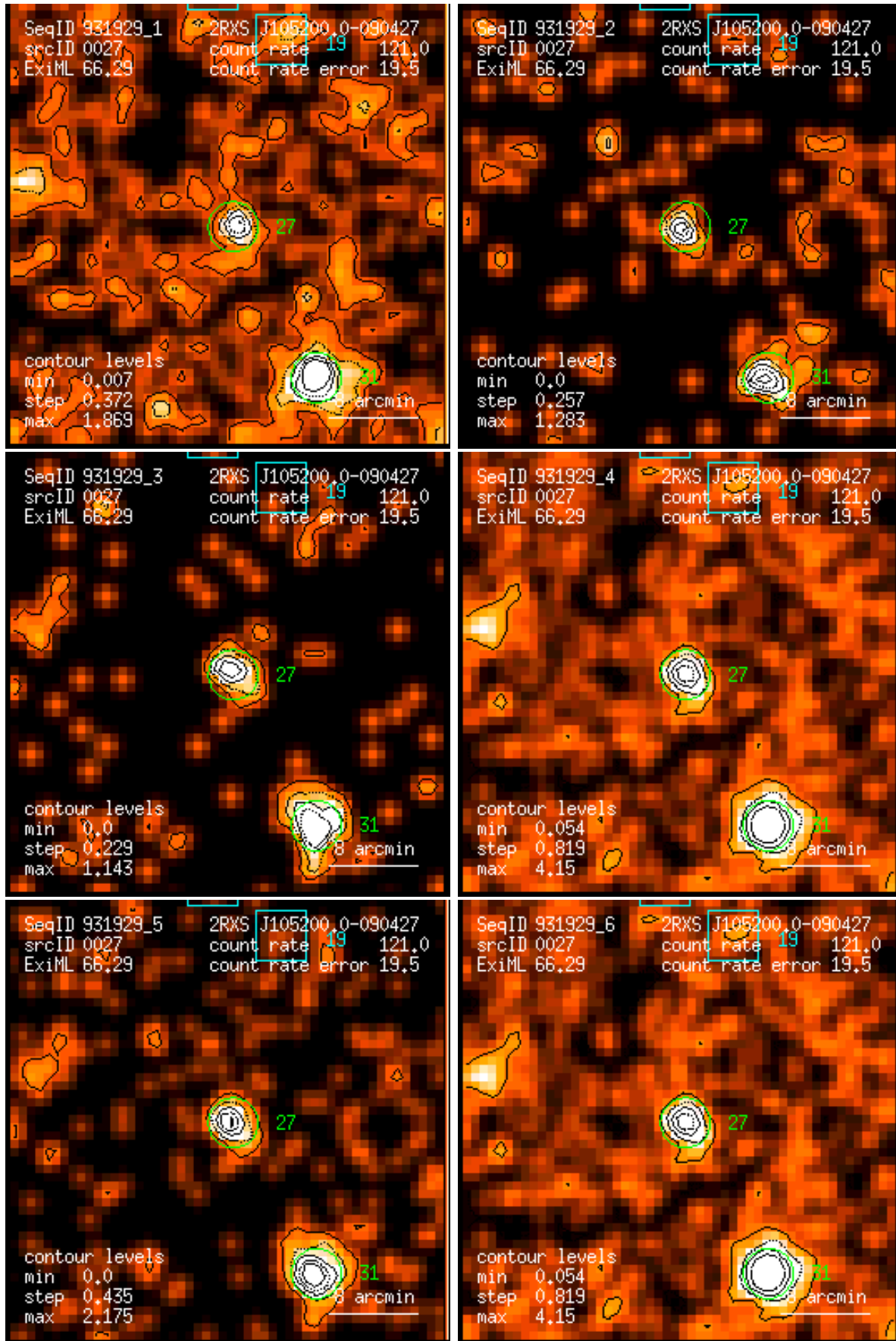
Figure 27: RASS 931929: detection 0027: band rate images, Gaussian filter: (1) PSPC channels 11 – 41, (2) 52 – 90, (3) 91 – 201, (4) 11 – 235, (5) 52 – 201, (6) 11 – 201. Broad band rates in counts/ks. Band rate contour levels in counts/ks/arcmin 2 .
