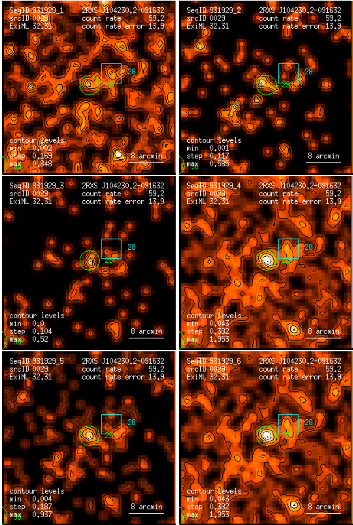
Figure 29: RASS 931929: detection 0029: band rate images, Gaussian filter: (1) PSPC channels 11 – 41, (2) 52 – 90, (3) 91 – 201, (4) 11 – 235, (5) 52 – 201, (6) 11 – 201. Broad band rates in counts/ks. Band rate contour levels in counts/ks/arcmin 2 .
