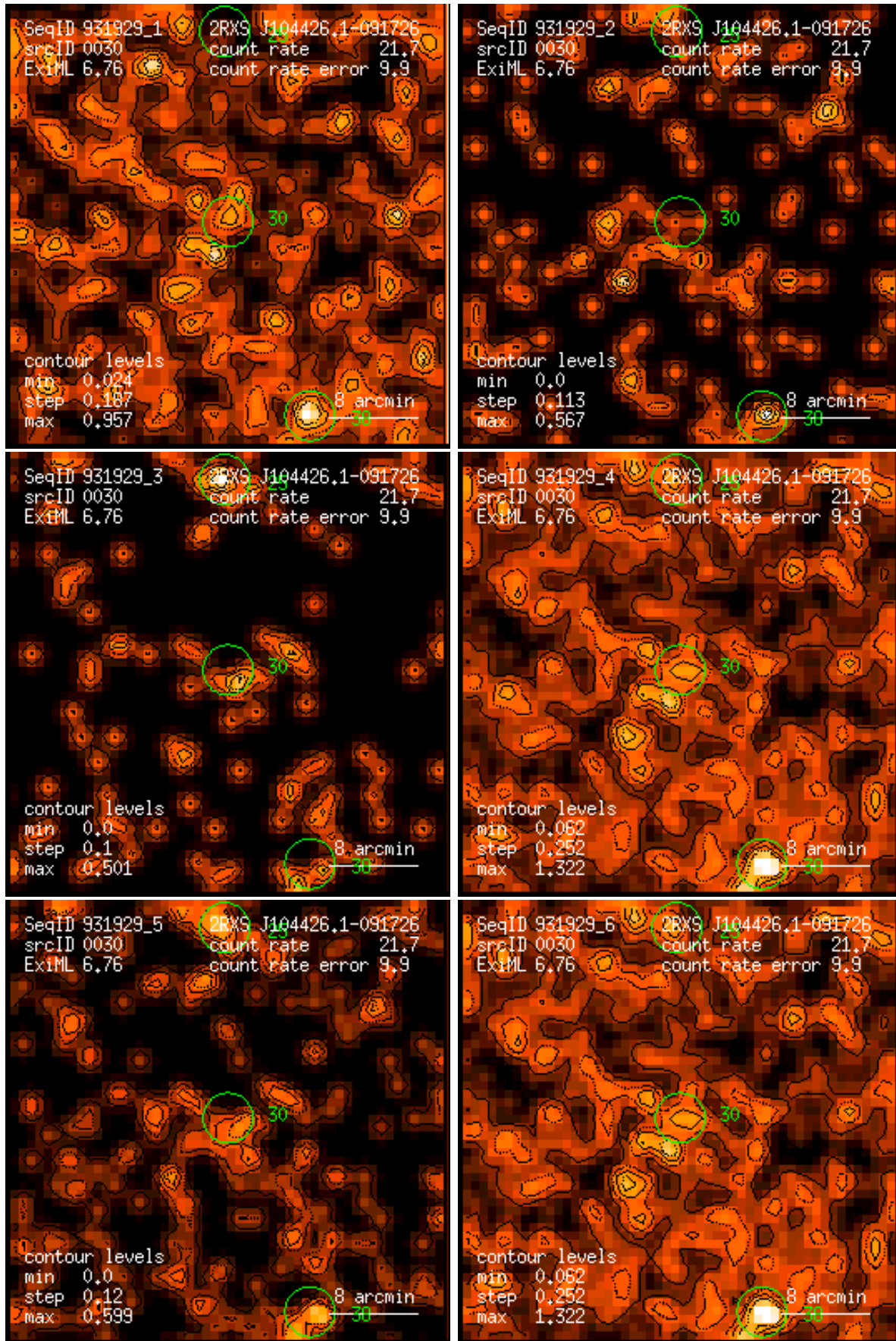
Figure 30: RASS 931929: detection 0030: band rate images, Gaussian filter: (1) PSPC channels 11 – 41, (2) 52 – 90, (3) 91 – 201, (4) 11 – 235, (5) 52 – 201, (6) 11 – 201. Broad band rates in counts/ks. Band rate contour levels in counts/ks/arcmin 2 .
