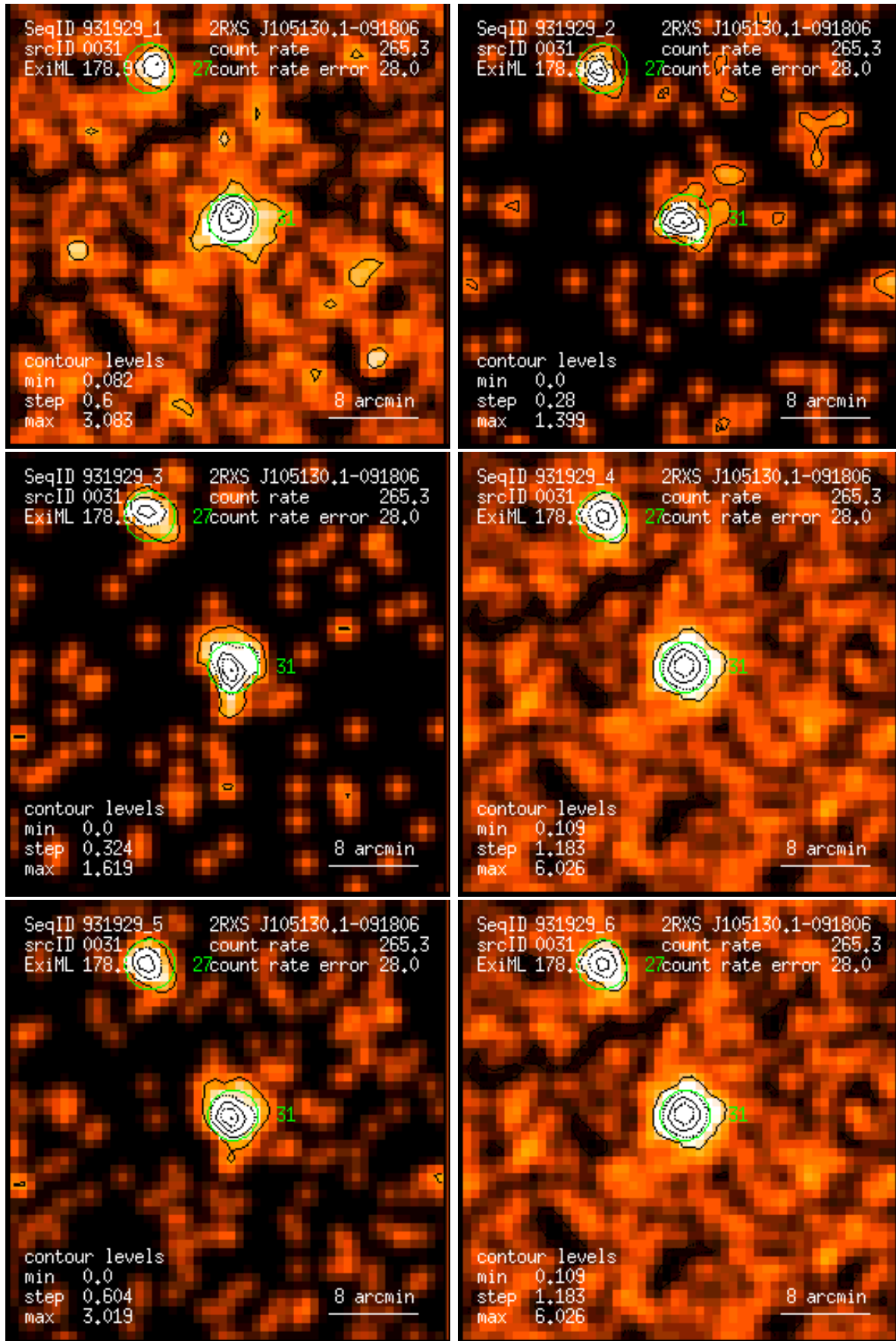
Figure 31: RASS 931929: detection 0031: band rate images, Gaussian filter: (1) PSPC channels 11 – 41, (2) 52 – 90, (3) 91 – 201, (4) 11 – 235, (5) 52 – 201, (6) 11 – 201. Broad band rates in counts/ks. Band rate contour levels in counts/ks/arcmin 2 .
