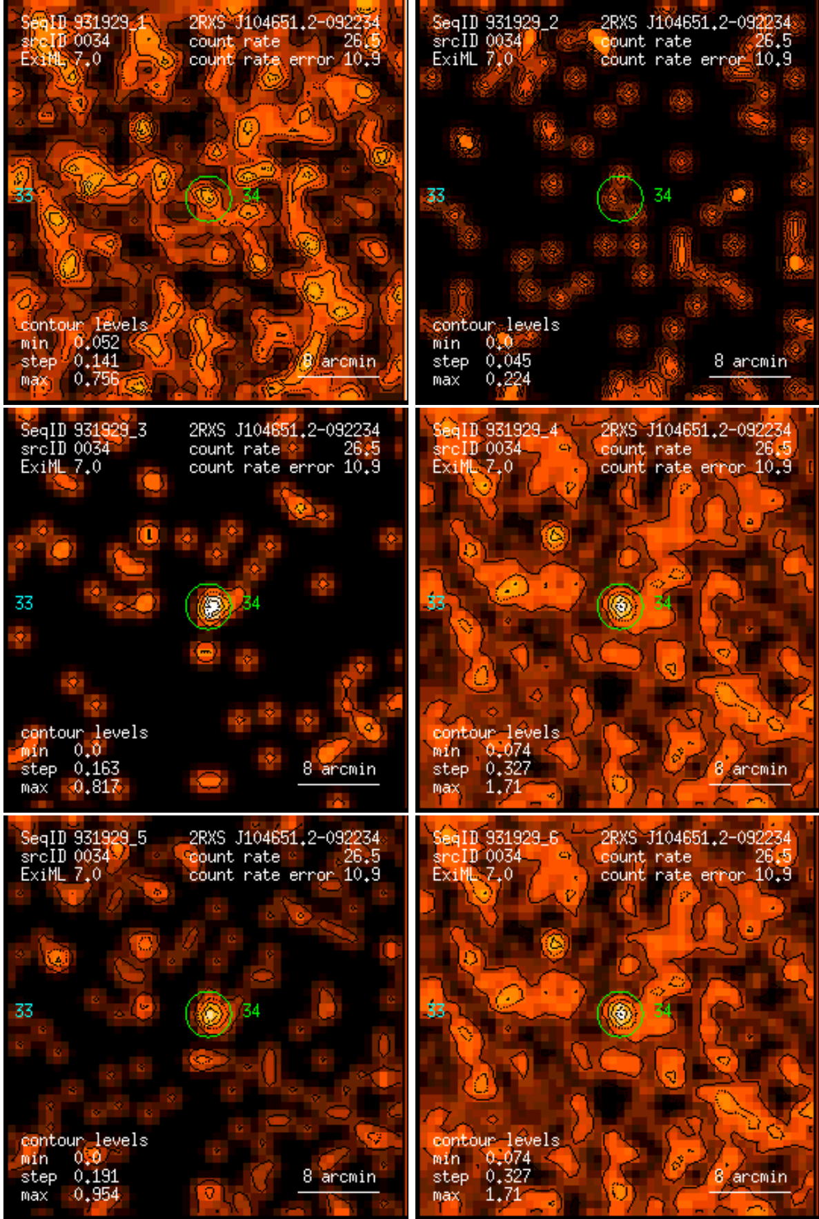
Figure 34: RASS 931929: detection 0034: band rate images, Gaussian filter: (1) PSPC channels 11 – 41, (2) 52 – 90, (3) 91 – 201, (4) 11 – 235, (5) 52 – 201, (6) 11 – 201. Broad band rates in counts/ks. Band rate contour levels in counts/ks/arcmin 2 .
