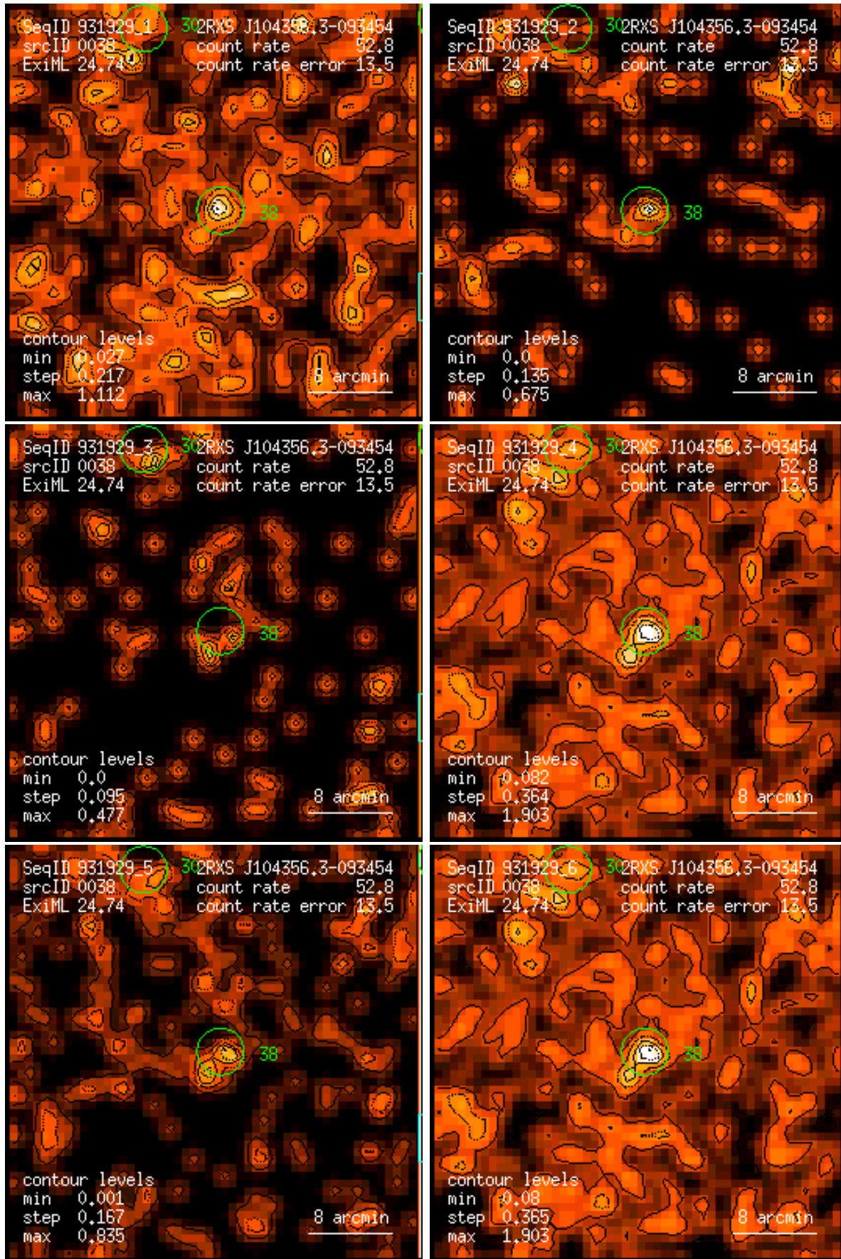
Figure 38: RASS 931929: detection 0038: band rate images, Gaussian filter: (1) PSPC channels 11 – 41, (2) 52 – 90, (3) 91 – 201, (4) 11 – 235, (5) 52 – 201, (6) 11 – 201. Broad band rates in counts/ks. Band rate contour levels in counts/ks/arcmin 2 .
