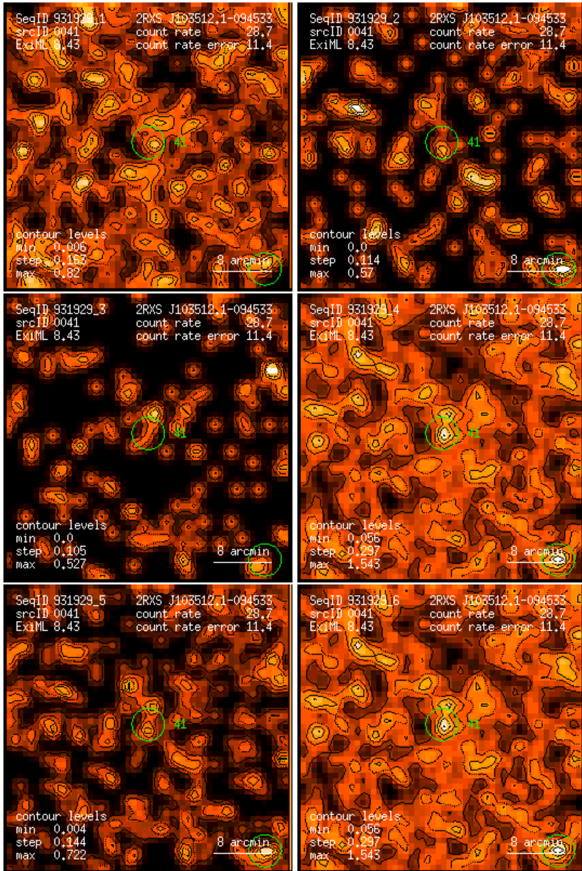
Figure 41: RASS 931929: detection 0041: band rate images, Gaussian filter: (1) PSPC channels 11 – 41, (2) 52 – 90, (3) 91 – 201, (4) 11 – 235, (5) 52 – 201, (6) 11 – 201. Broad band rates in counts/ks. Band rate contour levels in counts/ks/arcmin 2 .
