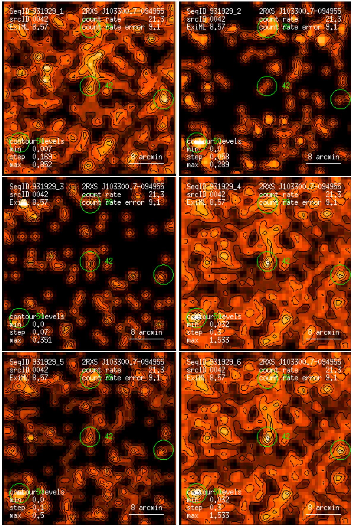
Figure 42: RASS 931929: detection 0042: band rate images, Gaussian filter: (1) PSPC channels 11 – 41, (2) 52 – 90, (3) 91 – 201, (4) 11 – 235, (5) 52 – 201, (6) 11 – 201. Broad band rates in counts/ks. Band rate contour levels in counts/ks/arcmin 2 .
