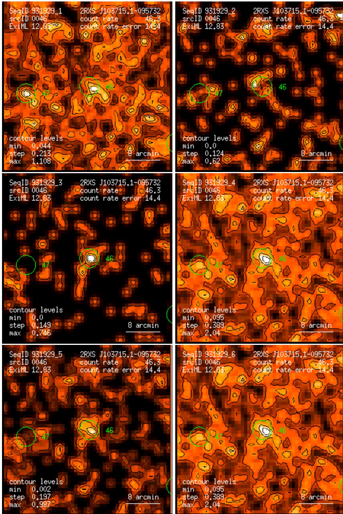
Figure 46: RASS 931929: detection 0046: band rate images, Gaussian filter: (1) PSPC channels 11 – 41, (2) 52 – 90, (3) 91 – 201, (4) 11 – 235, (5) 52 – 201, (6) 11 – 201. Broad band rates in counts/ks. Band rate contour levels in counts/ks/arcmin 2 .
