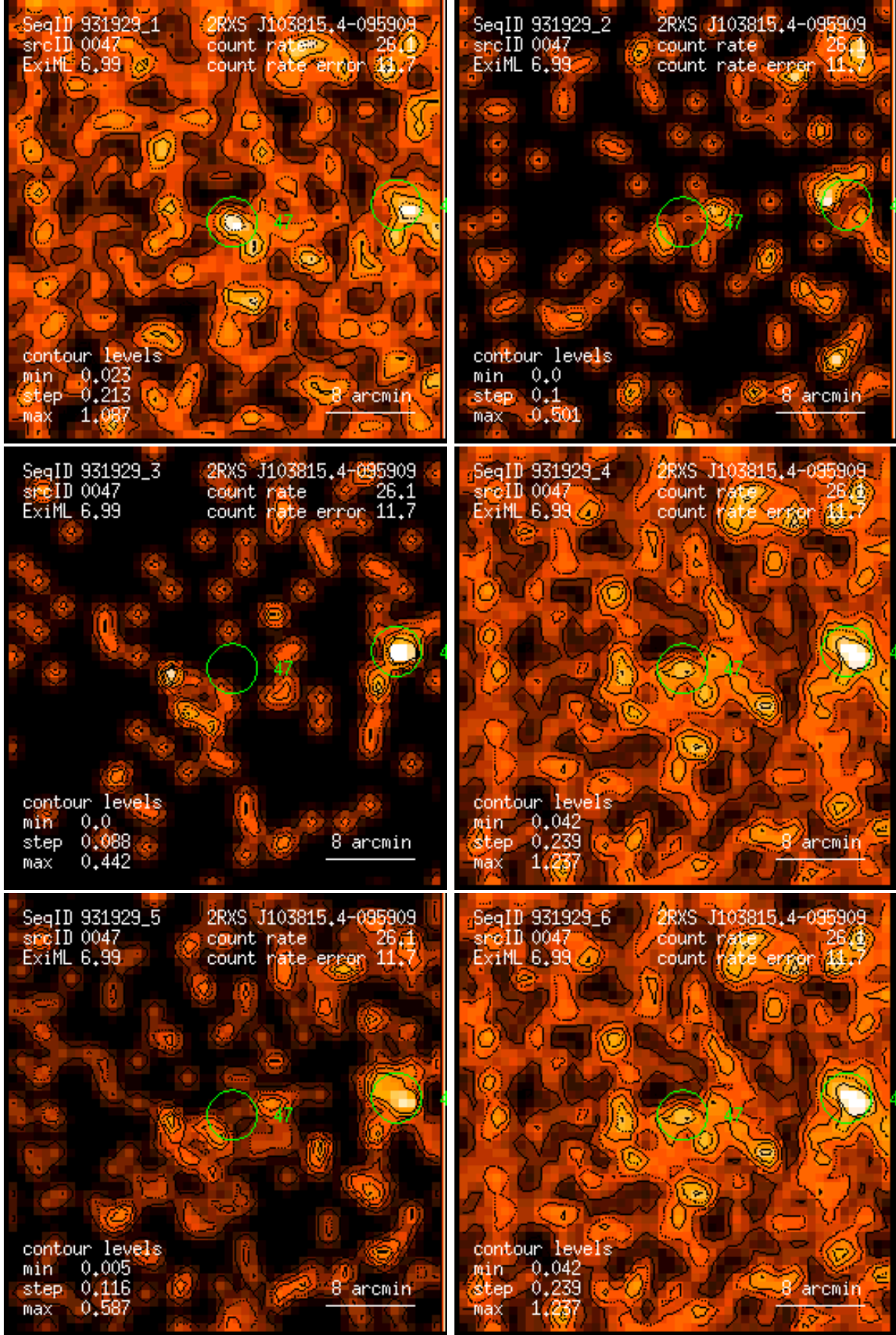
Figure 47: RASS 931929: detection 0047: band rate images, Gaussian filter: (1) PSPC channels 11 – 41, (2) 52 – 90, (3) 91 – 201, (4) 11 – 235, (5) 52 – 201, (6) 11 – 201. Broad band rates in counts/ks. Band rate contour levels in counts/ks/arcmin 2 .
