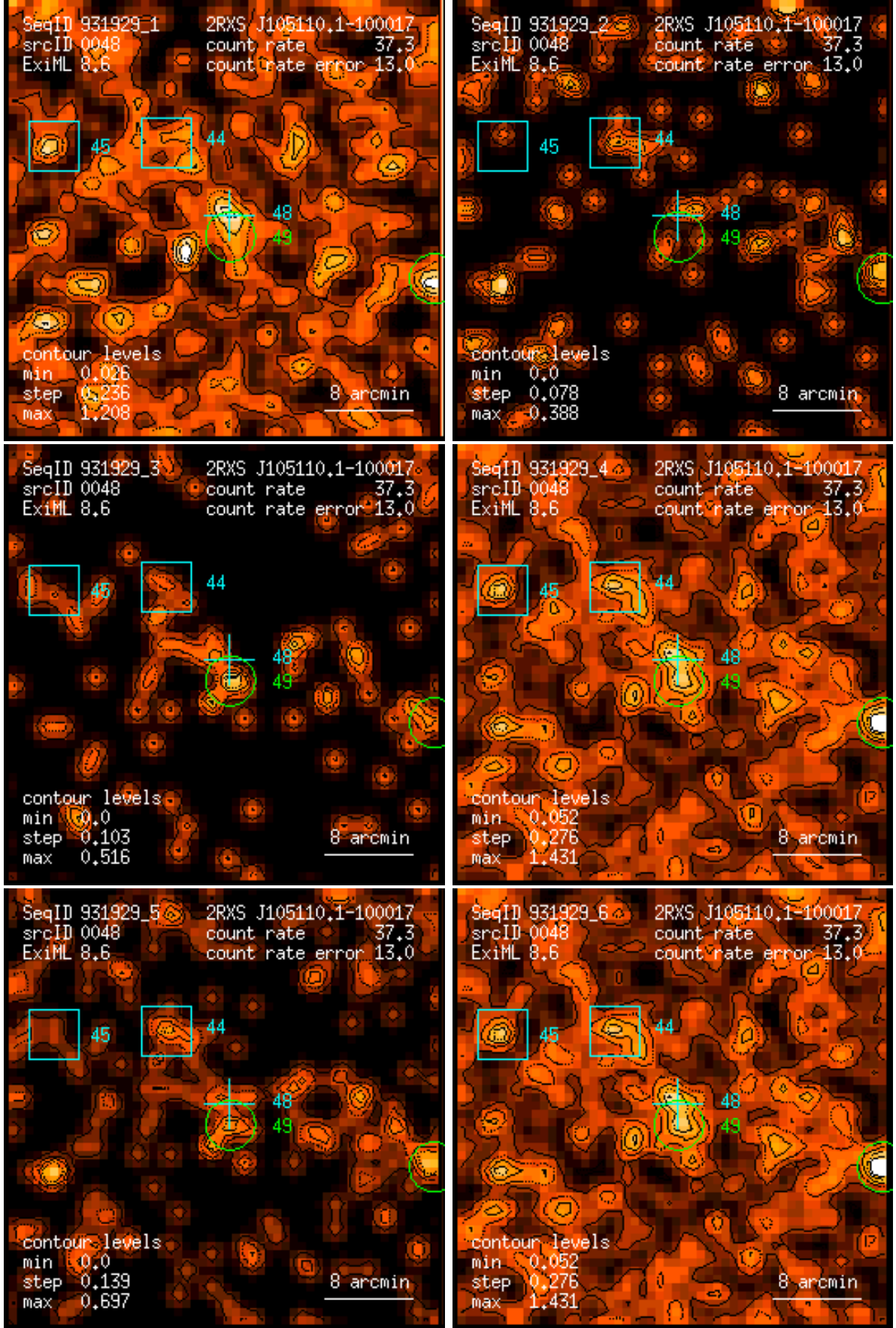
Figure 48: RASS 931929: detection 0048: band rate images, Gaussian filter: (1) PSPC channels 11 – 41, (2) 52 – 90, (3) 91 – 201, (4) 11 – 235, (5) 52 – 201, (6) 11 – 201. Broad band rates in counts/ks. Band rate contour levels in counts/ks/arcmin 2 .
