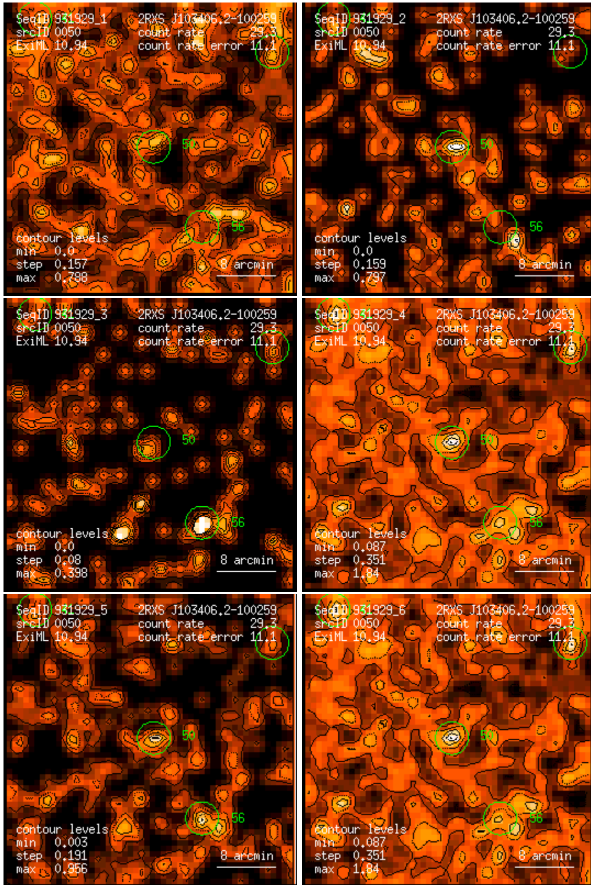
Figure 50: RASS 931929: detection 0050: band rate images, Gaussian filter: (1) PSPC channels 11 – 41, (2) 52 – 90, (3) 91 – 201, (4) 11 – 235, (5) 52 – 201, (6) 11 – 201. Broad band rates in counts/ks. Band rate contour levels in counts/ks/arcmin 2 .
