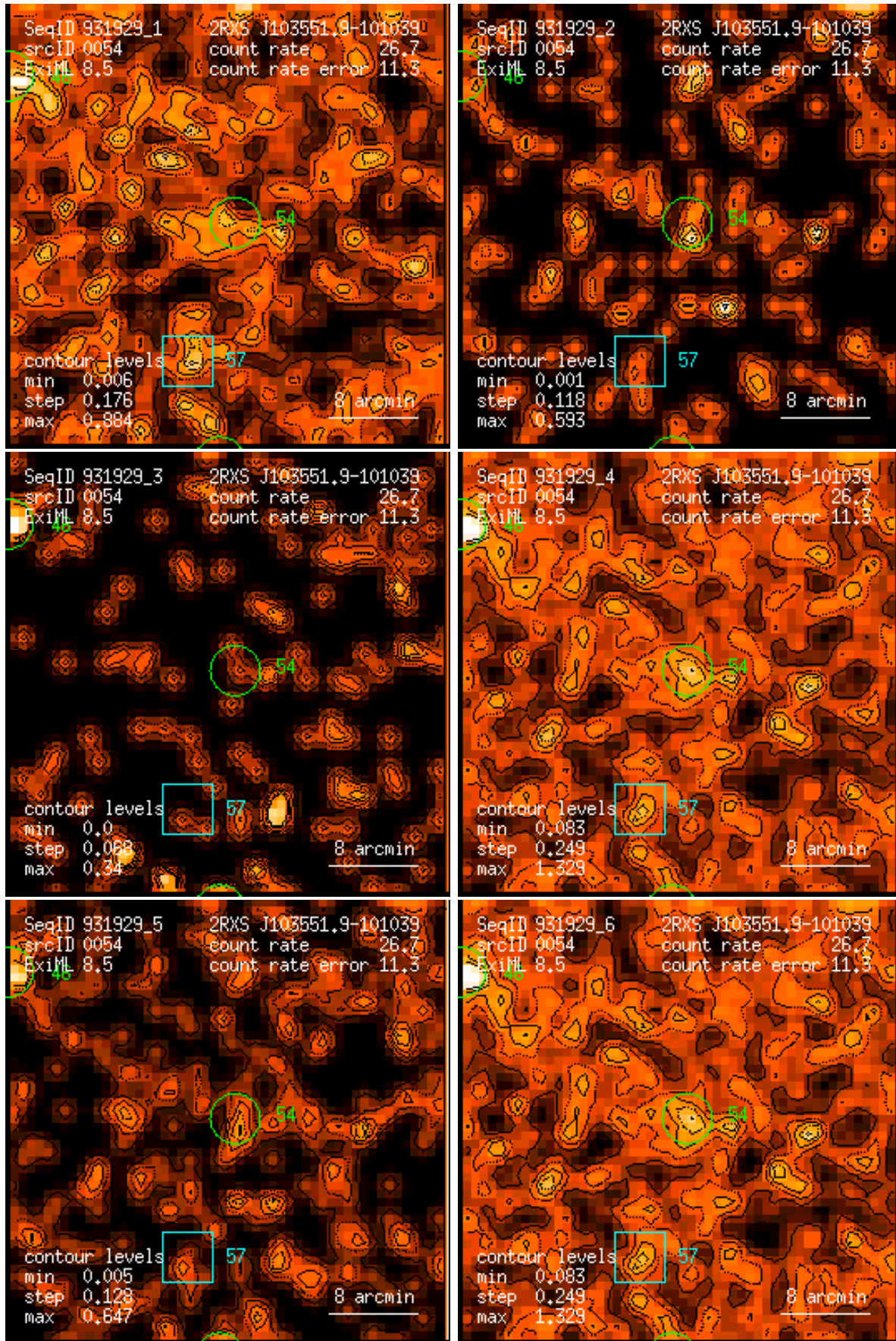
Figure 54: RASS 931929: detection 0054: band rate images, Gaussian filter: (1) PSPC channels 11 – 41, (2) 52 – 90, (3) 91 – 201, (4) 11 – 235, (5) 52 – 201, (6) 11 – 201. Broad band rates in counts/ks. Band rate contour levels in counts/ks/arcmin 2 .
