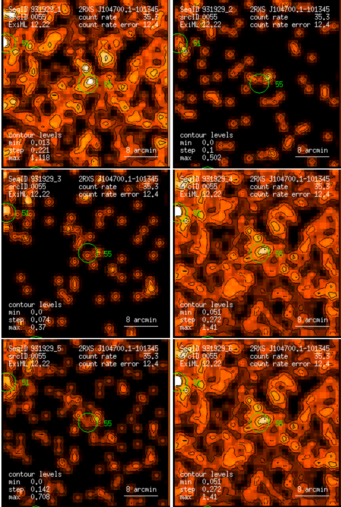
Figure 55: RASS 931929: detection 0055: band rate images, Gaussian filter: (1) PSPC channels 11 – 41, (2) 52 – 90, (3) 91 – 201, (4) 11 – 235, (5) 52 – 201, (6) 11 – 201. Broad band rates in counts/ks. Band rate contour levels in counts/ks/arcmin 2 .
