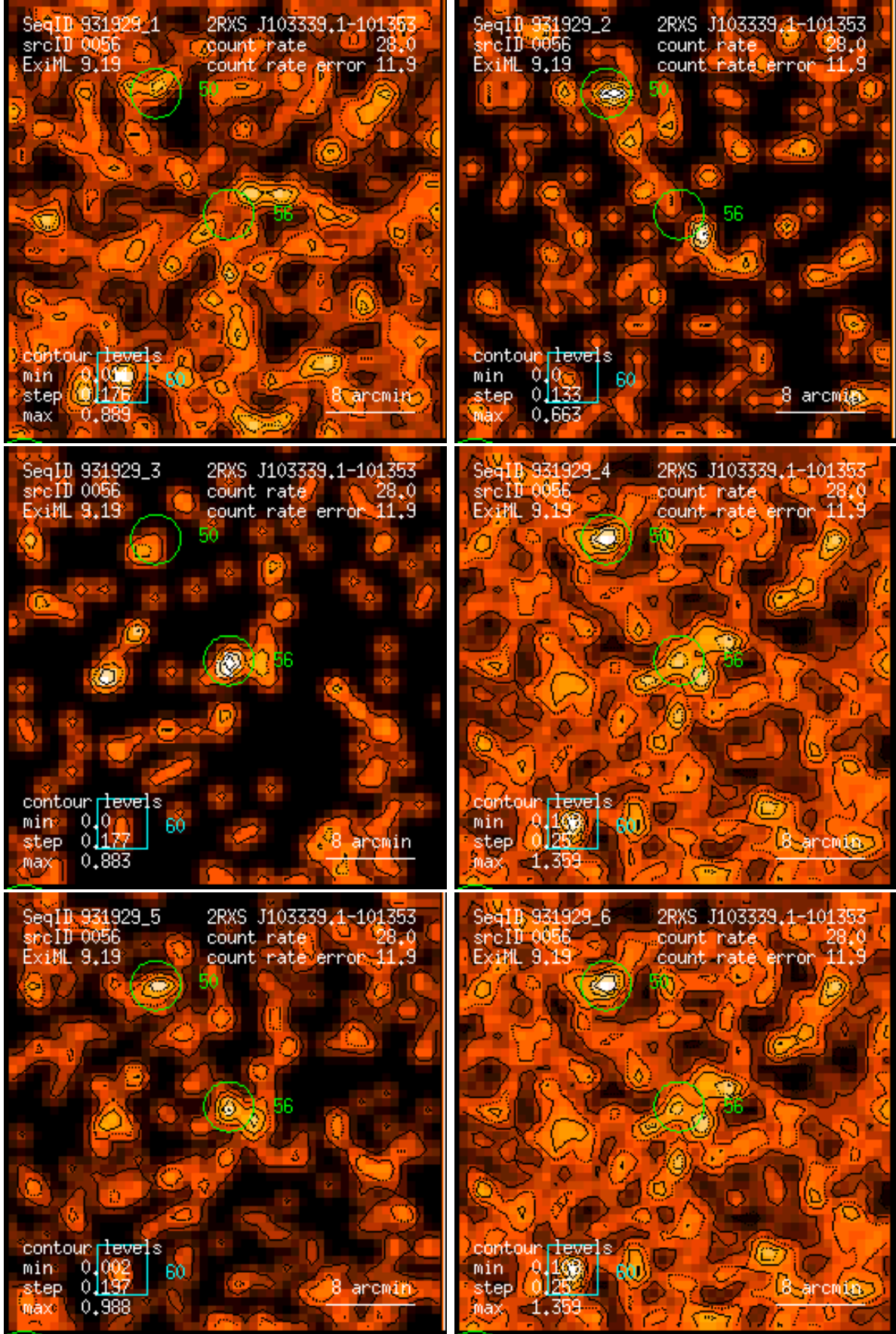
Figure 56: RASS 931929: detection 0056: band rate images, Gaussian filter: (1) PSPC channels 11 – 41, (2) 52 – 90, (3) 91 – 201, (4) 11 – 235, (5) 52 – 201, (6) 11 – 201. Broad band rates in counts/ks. Band rate contour levels in counts/ks/arcmin 2 .
