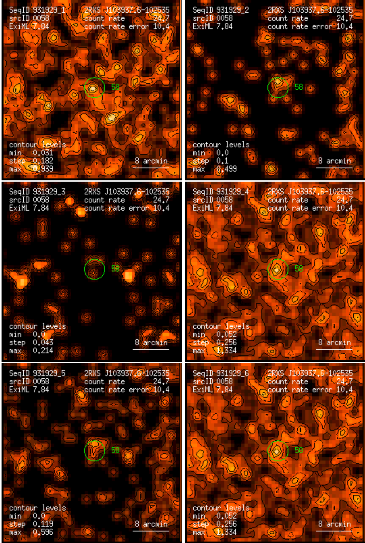
Figure 58: RASS 931929: detection 0058: band rate images, Gaussian filter: (1) PSPC channels 11 – 41, (2) 52 – 90, (3) 91 – 201, (4) 11 – 235, (5) 52 – 201, (6) 11 – 201. Broad band rates in counts/ks. Band rate contour levels in counts/ks/arcmin 2 .
