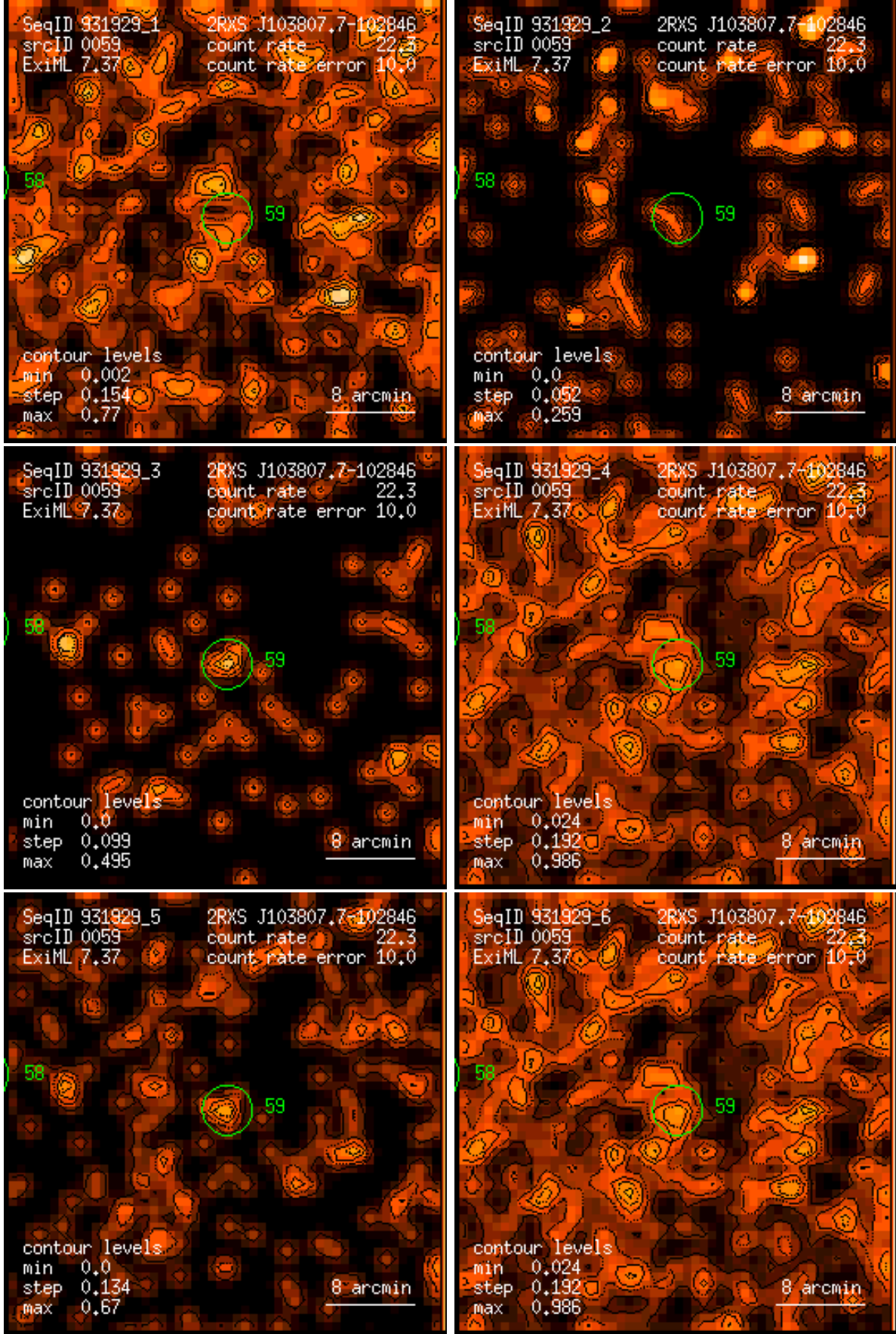
Figure 59: RASS 931929: detection 0059: band rate images, Gaussian filter: (1) PSPC channels 11 – 41, (2) 52 – 90, (3) 91 – 201, (4) 11 – 235, (5) 52 – 201, (6) 11 – 201. Broad band rates in counts/ks. Band rate contour levels in counts/ks/arcmin 2 .
