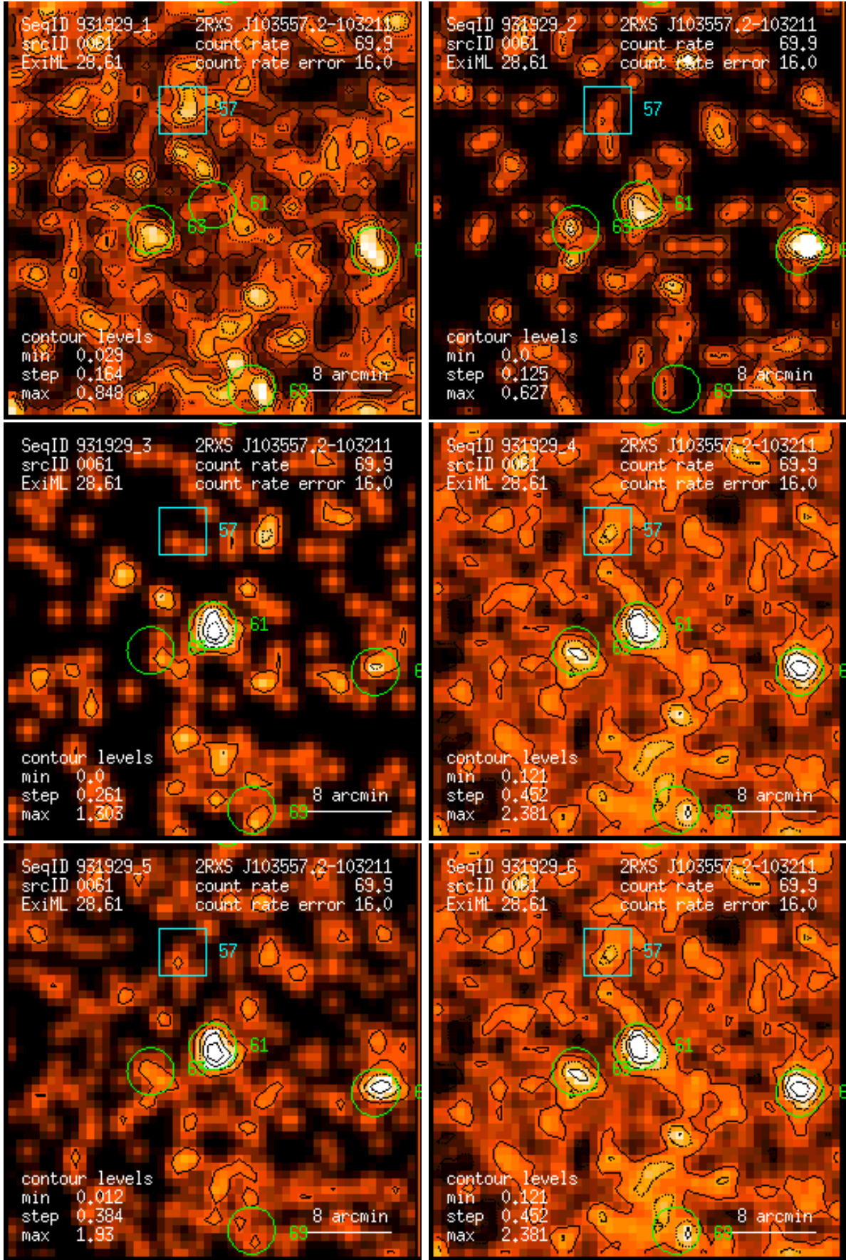
Figure 61: RASS 931929: detection 0061: band rate images, Gaussian filter: (1) PSPC channels 11 – 41, (2) 52 – 90, (3) 91 – 201, (4) 11 – 235, (5) 52 – 201, (6) 11 – 201. Broad band rates in counts/ks. Band rate contour levels in counts/ks/arcmin 2 .
