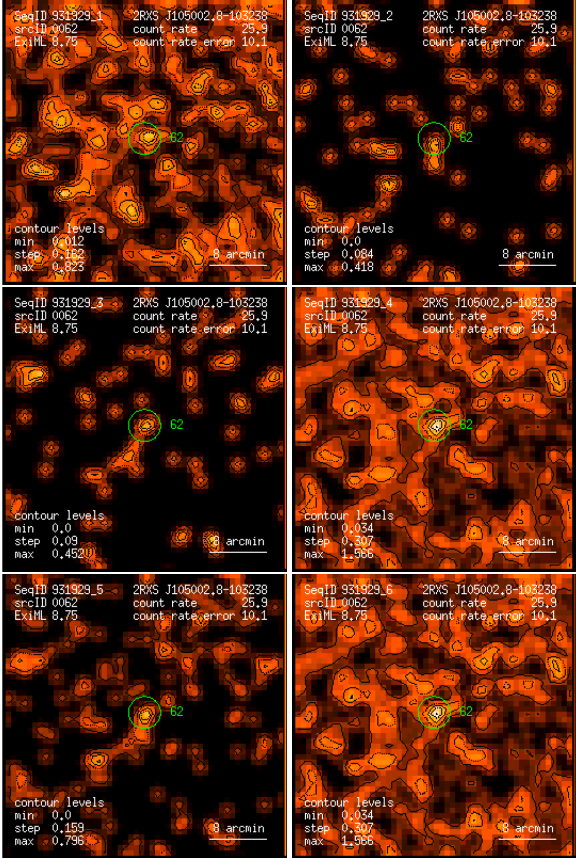
Figure 62: RASS 931929: detection 0062: band rate images, Gaussian filter: (1) PSPC channels 11 – 41, (2) 52 – 90, (3) 91 – 201, (4) 11 – 235, (5) 52 – 201, (6) 11 – 201. Broad band rates in counts/ks. Band rate contour levels in counts/ks/arcmin 2 .
