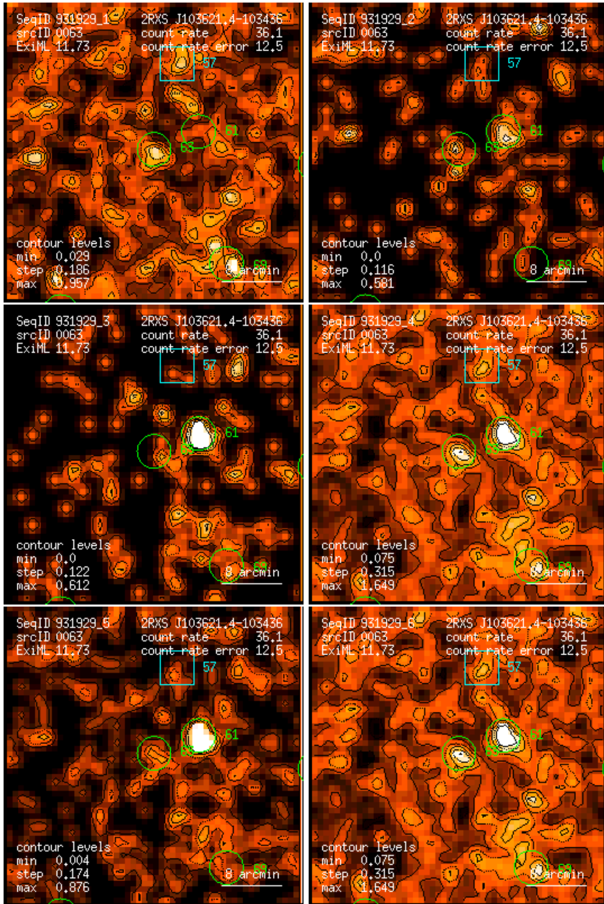
Figure 63: RASS 931929: detection 0063: band rate images, Gaussian filter: (1) PSPC channels 11 – 41, (2) 52 – 90, (3) 91 – 201, (4) 11 – 235, (5) 52 – 201, (6) 11 – 201. Broad band rates in counts/ks. Band rate contour levels in counts/ks/arcmin 2 .
