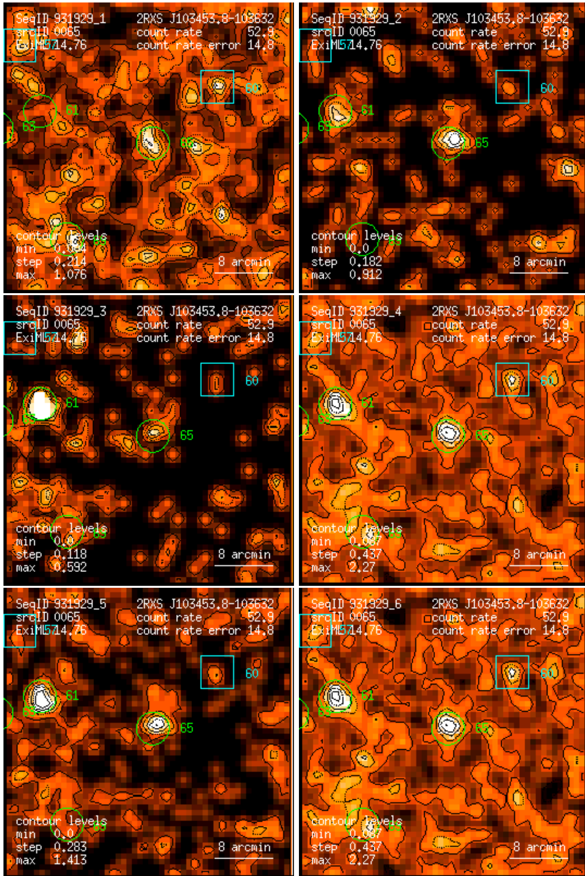
Figure 65: RASS 931929: detection 0065: band rate images, Gaussian filter: (1) PSPC channels 11 – 41, (2) 52 – 90, (3) 91 – 201, (4) 11 – 235, (5) 52 – 201, (6) 11 – 201. Broad band rates in counts/ks. Band rate contour levels in counts/ks/arcmin 2 .
