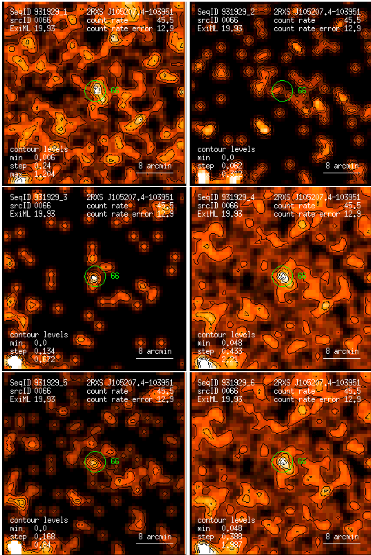
Figure 66: RASS 931929: detection 0066: band rate images, Gaussian filter: (1) PSPC channels 11 – 41, (2) 52 – 90, (3) 91 – 201, (4) 11 – 235, (5) 52 – 201, (6) 11 – 201. Broad band rates in counts/ks. Band rate contour levels in counts/ks/arcmin 2 .
