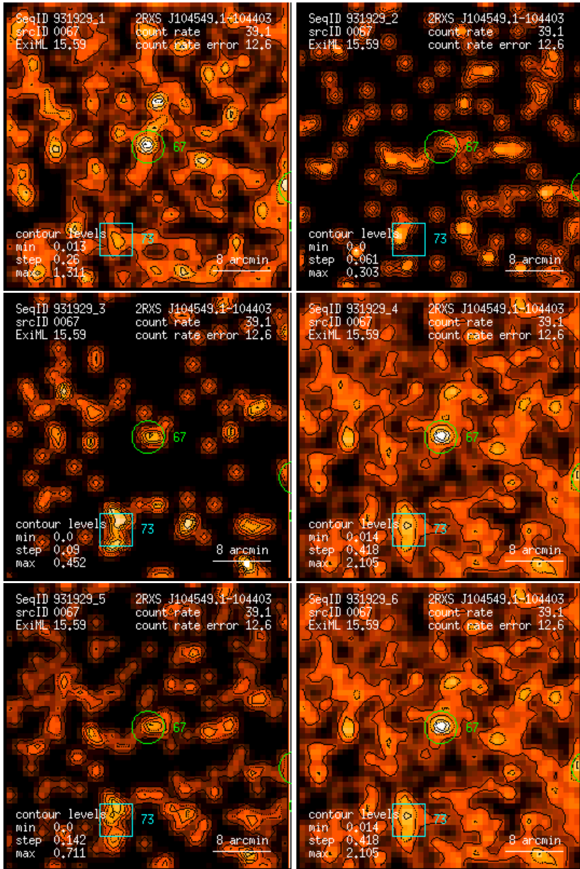
Figure 67: RASS 931929: detection 0067: band rate images, Gaussian filter: (1) PSPC channels 11 – 41, (2) 52 – 90, (3) 91 – 201, (4) 11 – 235, (5) 52 – 201, (6) 11 – 201. Broad band rates in counts/ks. Band rate contour levels in counts/ks/arcmin 2 .
