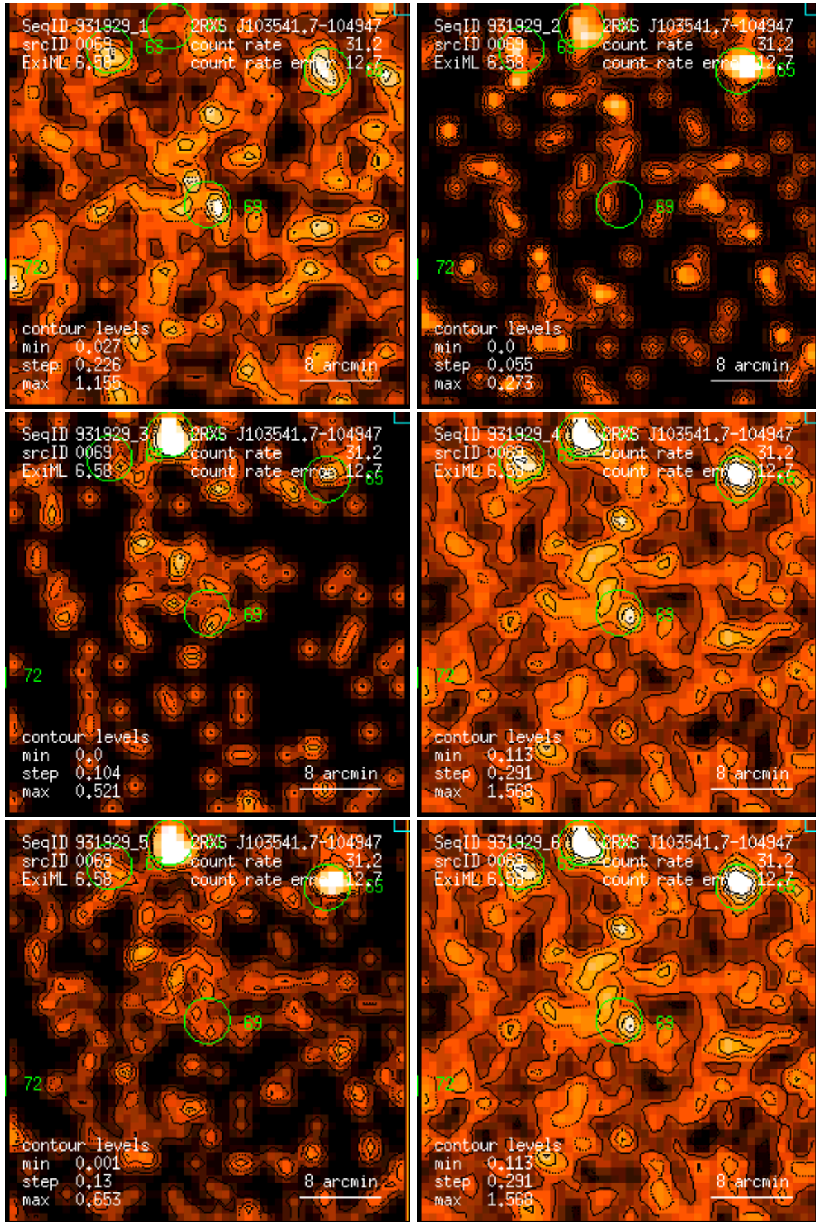
Figure 69: RASS 931929: detection 0069: band rate images, Gaussian filter: (1) PSPC channels 11 – 41, (2) 52 – 90, (3) 91 – 201, (4) 11 – 235, (5) 52 – 201, (6) 11 – 201. Broad band rates in counts/ks. Band rate contour levels in counts/ks/arcmin 2 .
