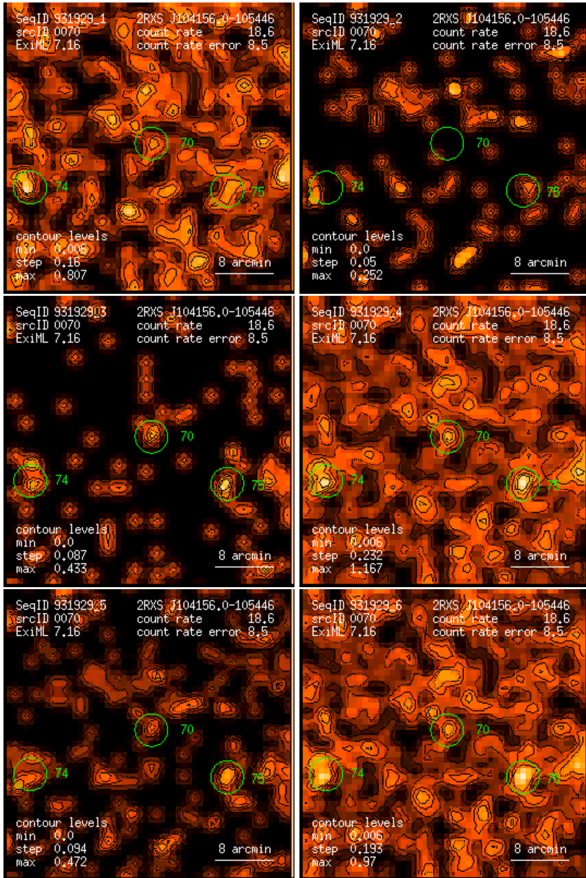
Figure 70: RASS 931929: detection 0070: band rate images, Gaussian filter: (1) PSPC channels 11 – 41, (2) 52 – 90, (3) 91 – 201, (4) 11 – 235, (5) 52 – 201, (6) 11 – 201. Broad band rates in counts/ks. Band rate contour levels in counts/ks/arcmin 2 .
