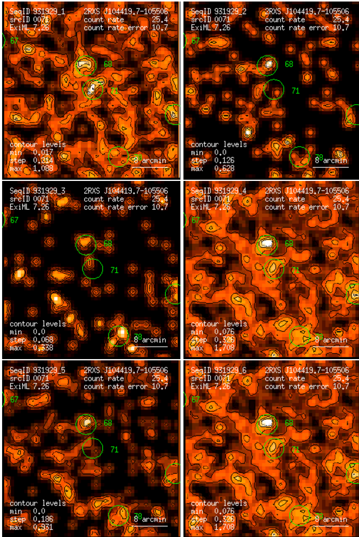
Figure 71: RASS 931929: detection 0071: band rate images, Gaussian filter: (1) PSPC channels 11 – 41, (2) 52 – 90, (3) 91 – 201, (4) 11 – 235, (5) 52 – 201, (6) 11 – 201. Broad band rates in counts/ks. Band rate contour levels in counts/ks/arcmin 2 .
