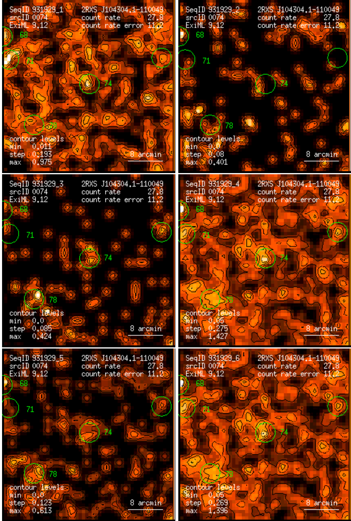
Figure 74: RASS 931929: detection 0074: band rate images, Gaussian filter: (1) PSPC channels 11 – 41, (2) 52 – 90, (3) 91 – 201, (4) 11 – 235, (5) 52 – 201, (6) 11 – 201. Broad band rates in counts/ks. Band rate contour levels in counts/ks/arcmin 2 .
