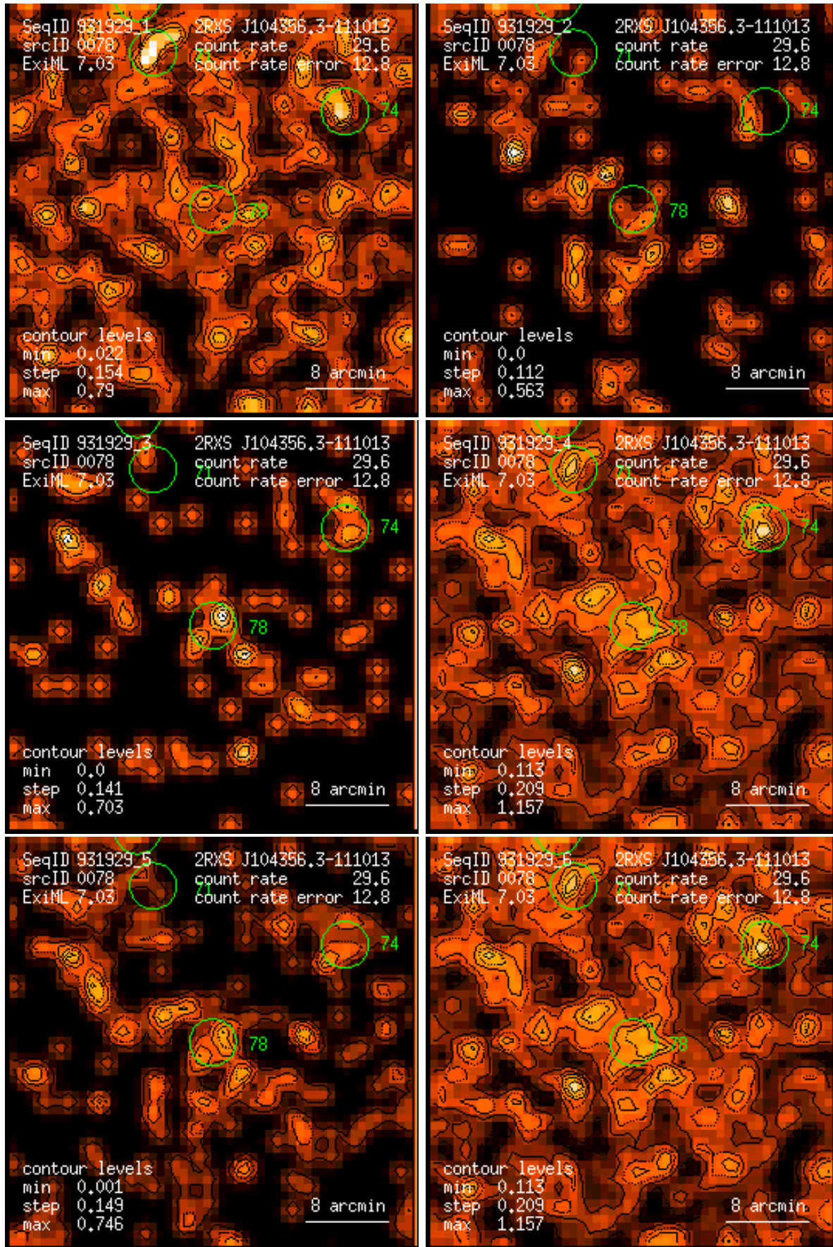
Figure 78: RASS 931929: detection 0078: band rate images, Gaussian filter: (1) PSPC channels 11 – 41, (2) 52 – 90, (3) 91 – 201, (4) 11 – 235, (5) 52 – 201, (6) 11 – 201. Broad band rates in counts/ks. Band rate contour levels in counts/ks/arcmin 2 .
