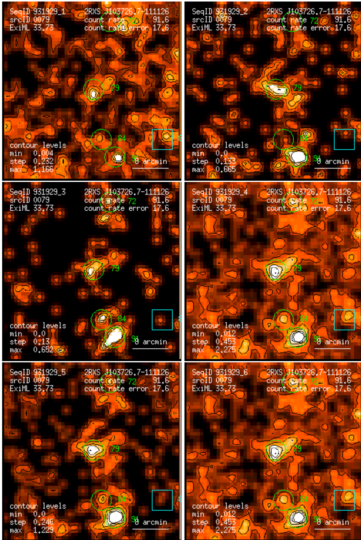
Figure 79: RASS 931929: detection 0079: band rate images, Gaussian filter: (1) PSPC channels 11 – 41, (2) 52 – 90, (3) 91 – 201, (4) 11 – 235, (5) 52 – 201, (6) 11 – 201. Broad band rates in counts/ks. Band rate contour levels in counts/ks/arcmin 2 .
