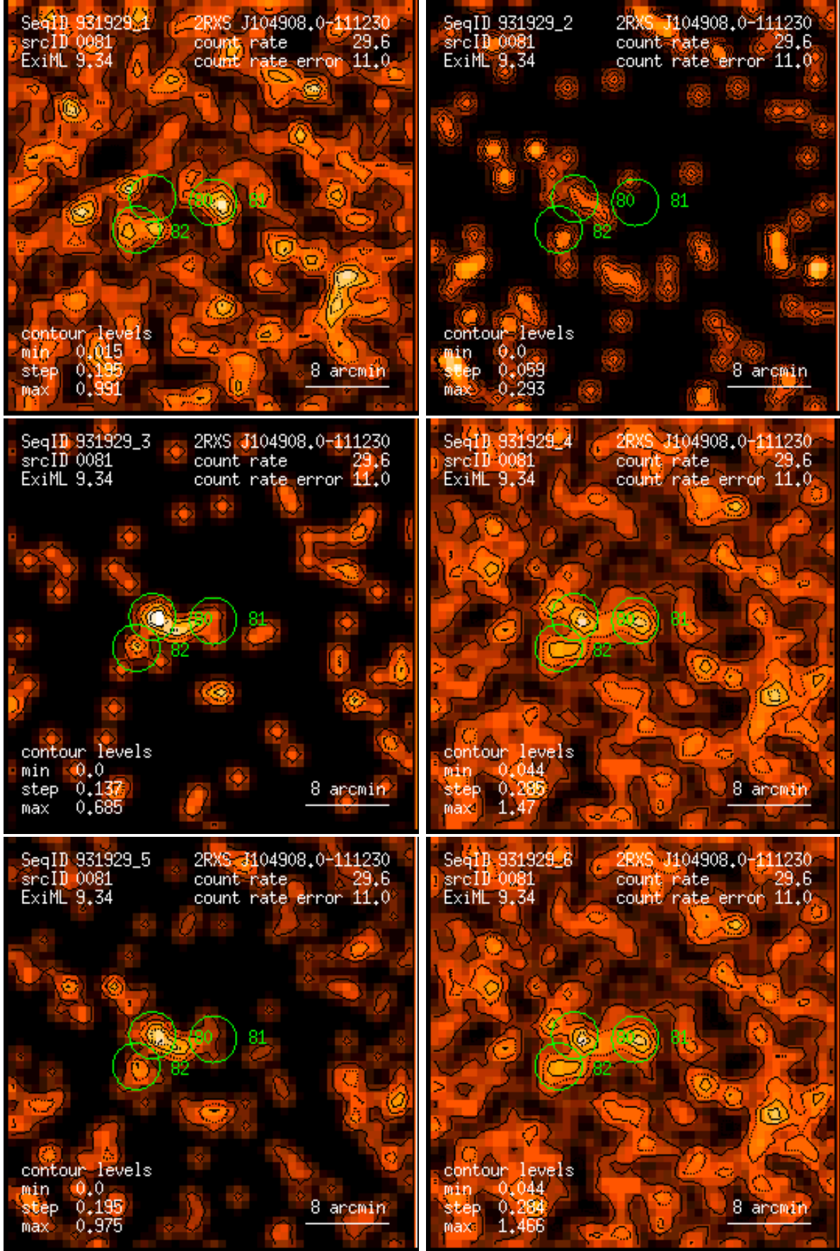
Figure 81: RASS 931929: detection 0081: band rate images, Gaussian filter: (1) PSPC channels 11 – 41, (2) 52 – 90, (3) 91 – 201, (4) 11 – 235, (5) 52 – 201, (6) 11 – 201. Broad band rates in counts/ks. Band rate contour levels in counts/ks/arcmin 2 .
