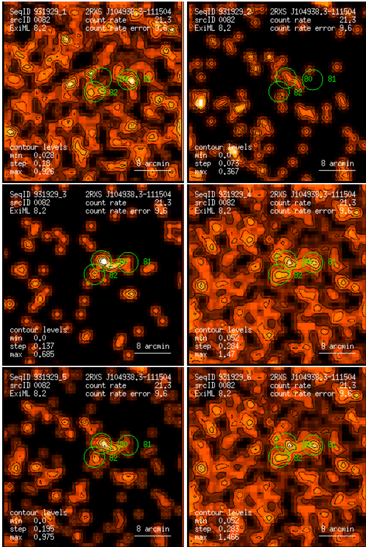
Figure 82: RASS 931929: detection 0082: band rate images, Gaussian filter: (1) PSPC channels 11 – 41, (2) 52 – 90, (3) 91 – 201, (4) 11 – 235, (5) 52 – 201, (6) 11 – 201. Broad band rates in counts/ks. Band rate contour levels in counts/ks/arcmin 2 .
